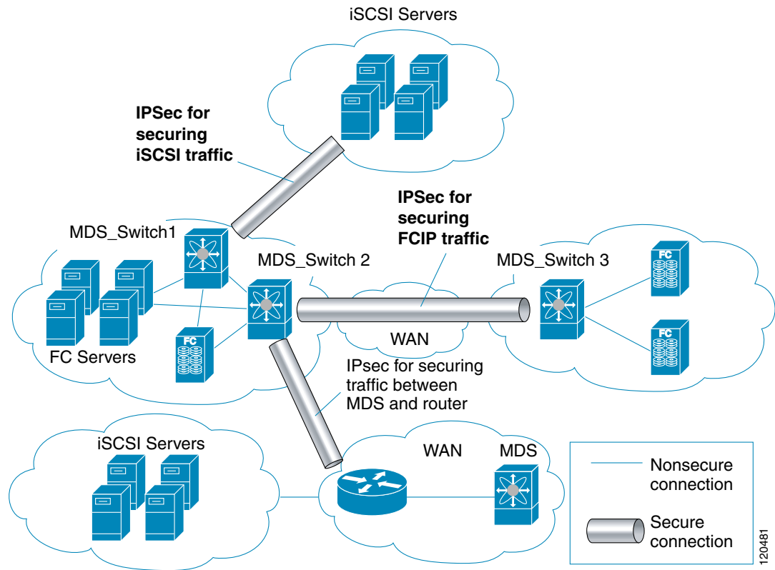
Figure 10-1 FCIP and iSCSI Scenarios Using MPS-14/2 Modules
