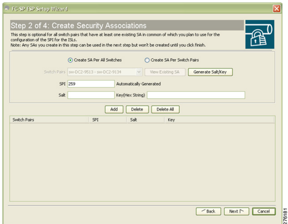
Figure 15-13 Create Security Associations
