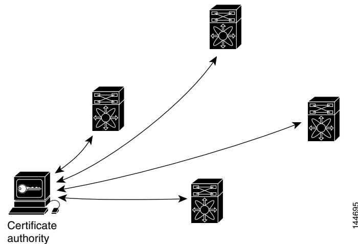
Figure 10-4 Dynamically Authenticating Devices with a CA
