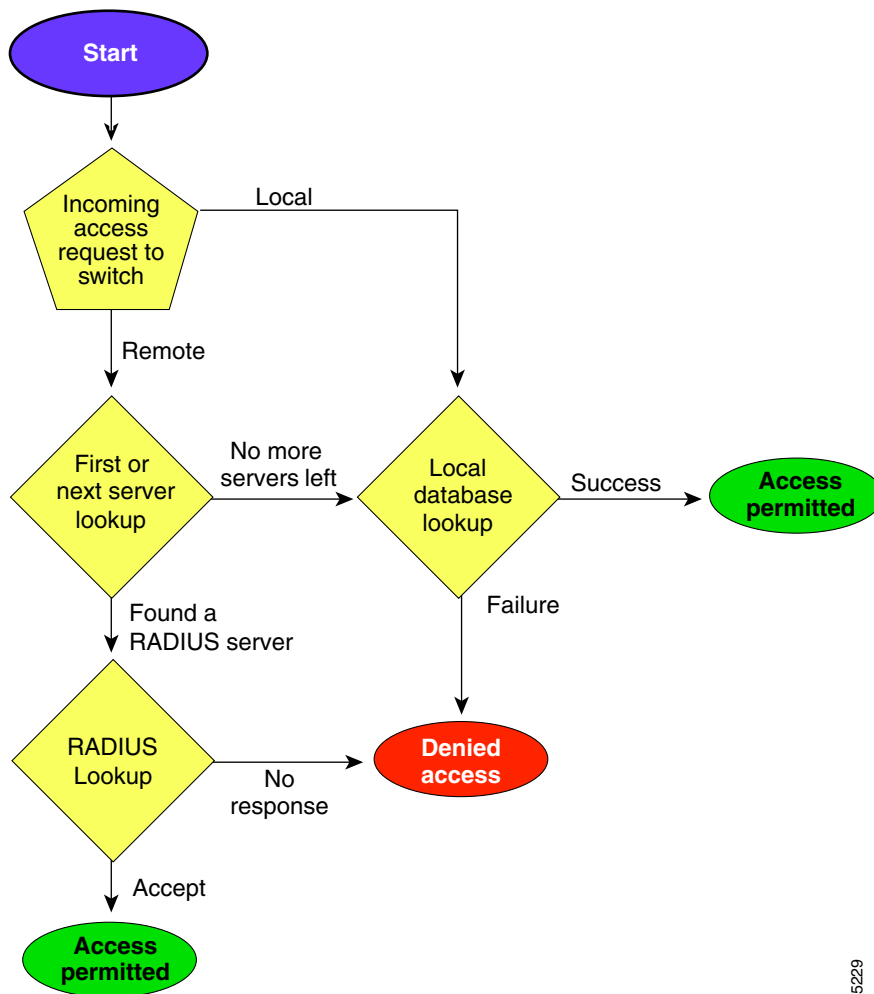
Figure 7-2 Switch Authorization and Authentication Flow
