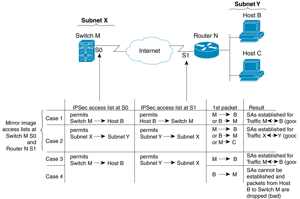
Figure 10-18 IPsec Processing of Mirror Image Configuration
