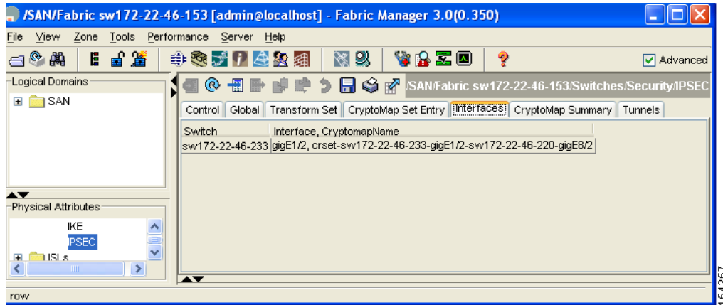
Figure 10-33 Crypto Map Interfaces
