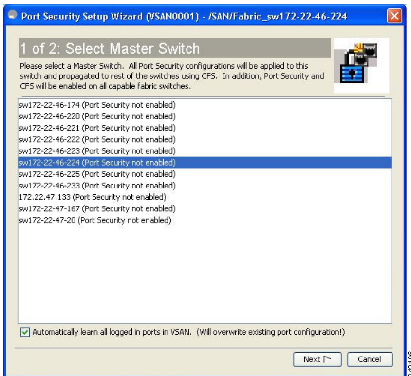
Figure 12-2 Select Master Switch Page
