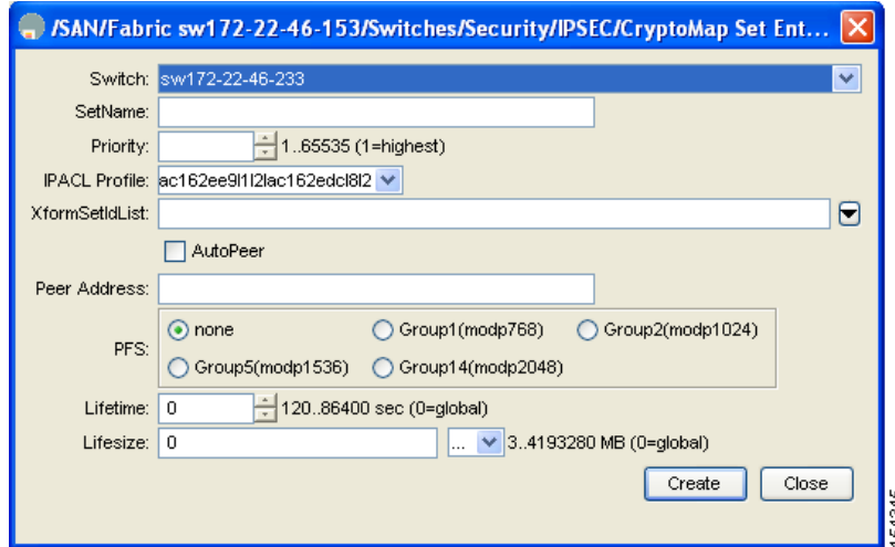
Figure 10-23 Create Crypto Map Dialog Box
