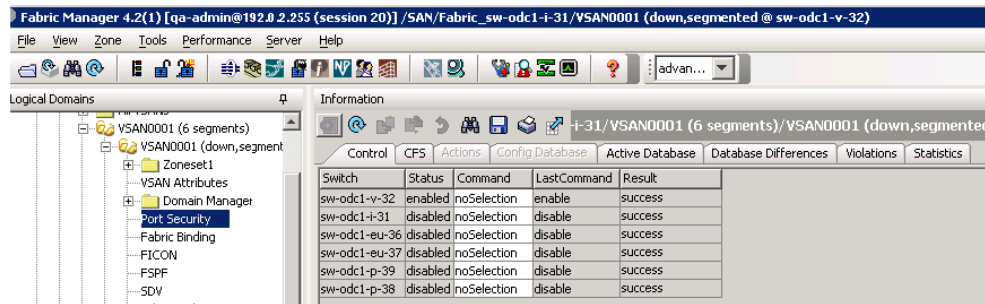
Figure 12-5 Port Security Configuration
