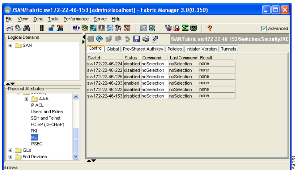
Figure 10-14 Create Initiator Version Dialog Box
