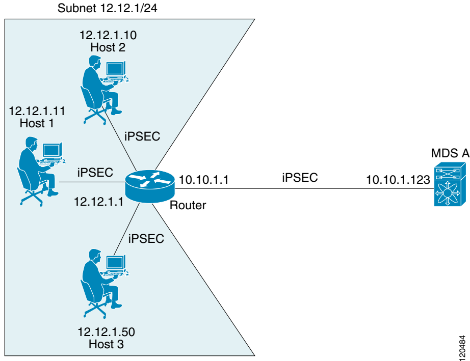
Figure 10-36 iSCSI with End-to-End IPsec
