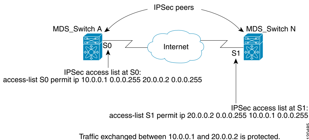
Figure 10-17 IPsec Processing of Crypto IPv4-ACLs
