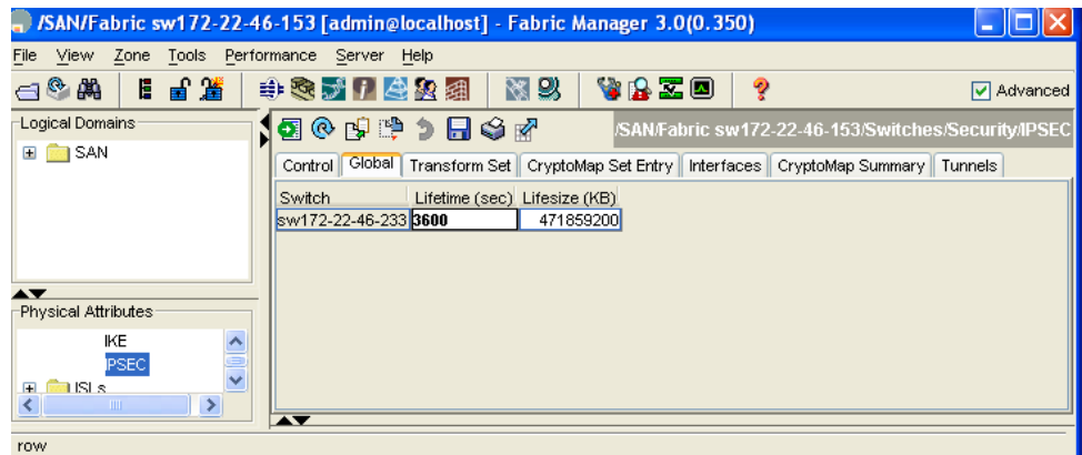
Figure 10-34 IPsec Configuration Global Tab
