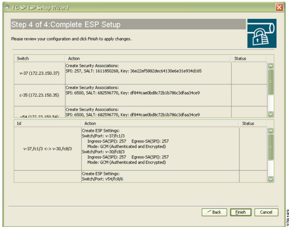
Figure 15-15 Complete ESP Setup
