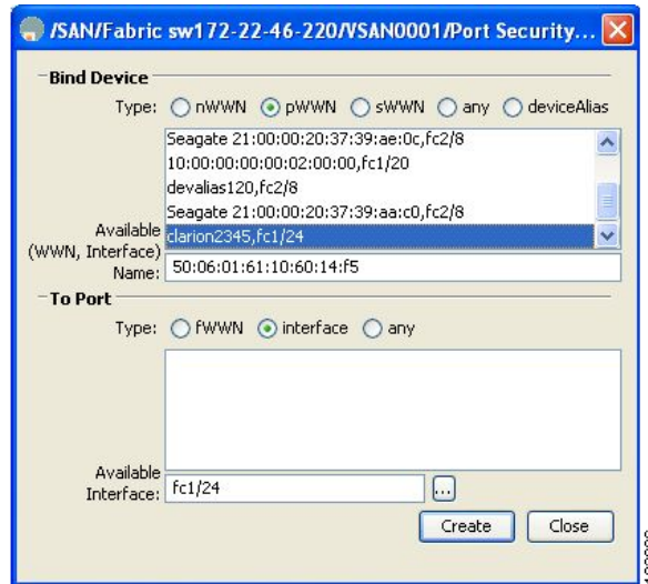
Figure 12-9 Create Port Security Dialog Box
