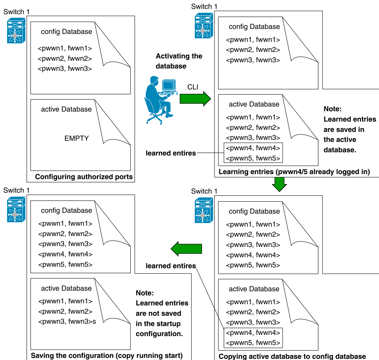
Figure 12-10 Port Security Database Scenarios
