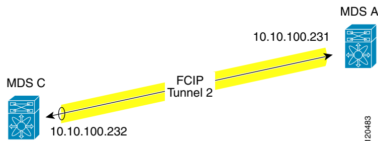
Figure 10-35 IP Security Usage in an FCIP Scenario
