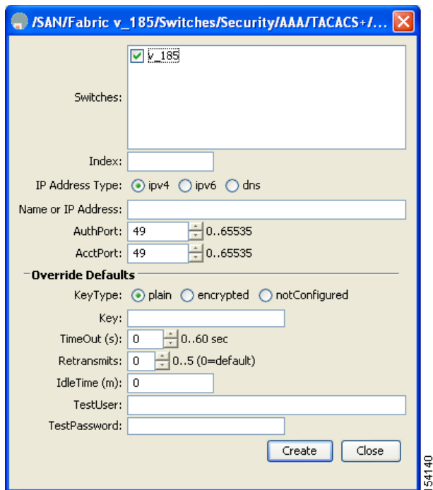
Figure 7-5 Create TACACS+ Server Dialog Box
