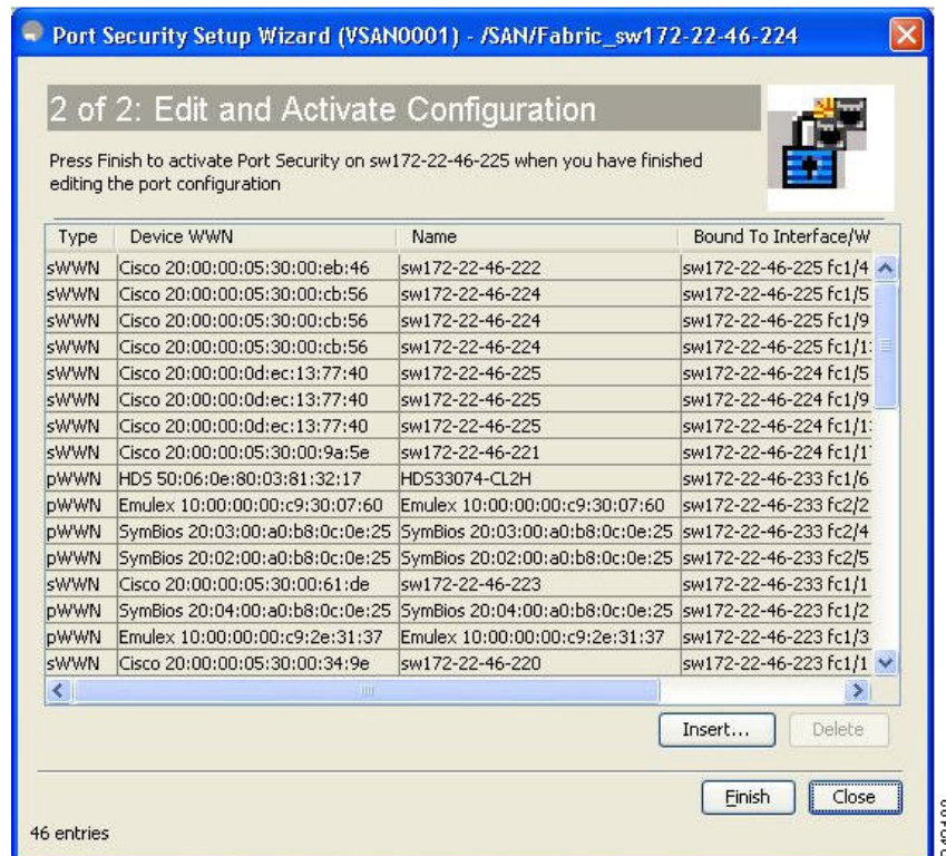
Figure 12-3 Edit and Activate Configuration Page
