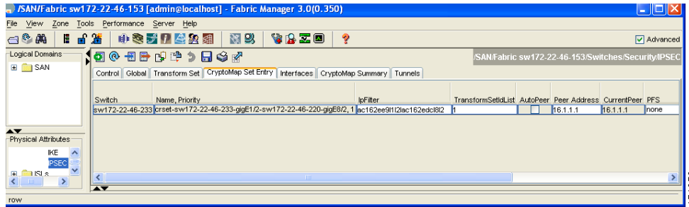
Figure 10-25 Existing Crypto Maps - Leftmost Columns
