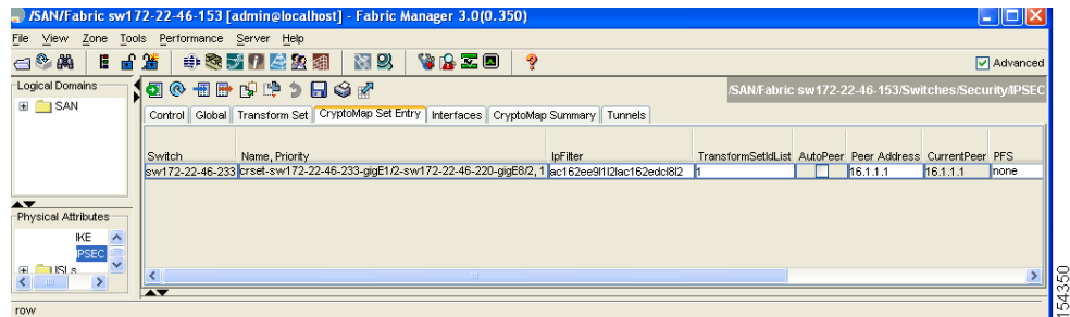
Figure 10-22 Existing Crypto Maps
