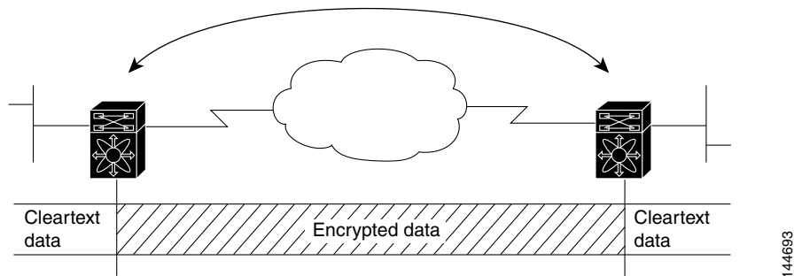
Figure 10-2 Two IPsec Switches Without CAs and Digital Certificates
