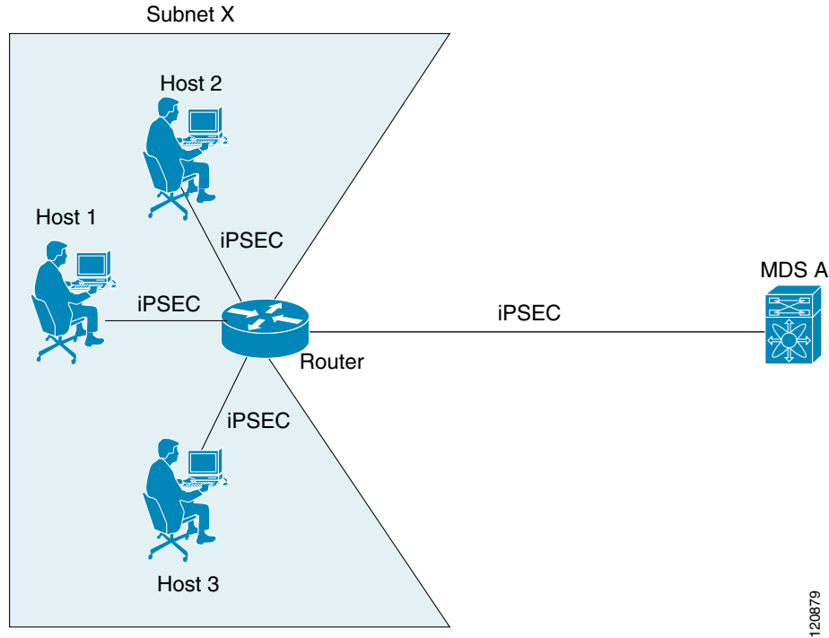
Figure 10-27 iSCSI with End-to-End IPsec Using the auto-peer Option
