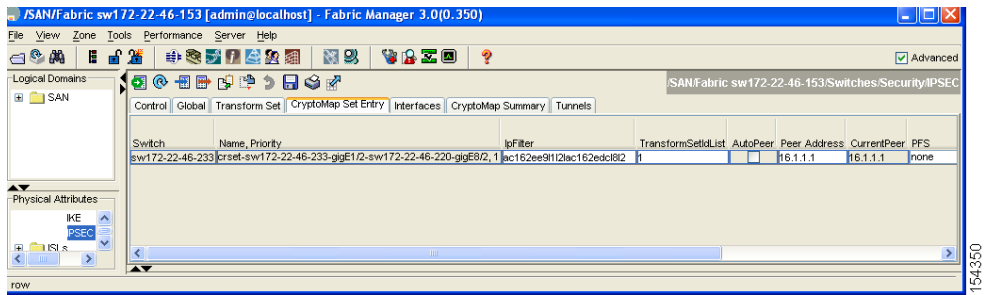
Figure 10-29 Existing Crypto Maps
