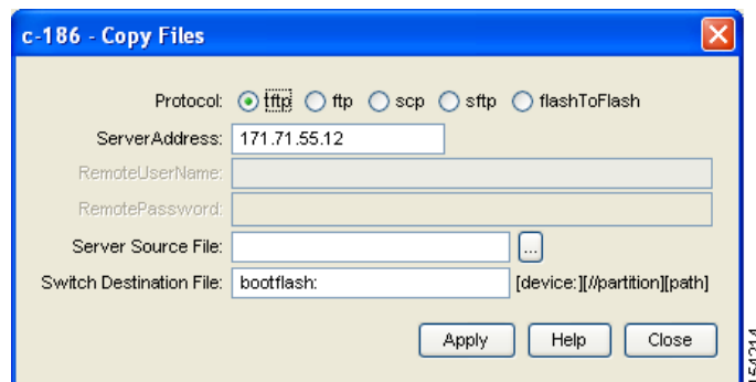
Figure 9-6 Copy Files Dialog Box
