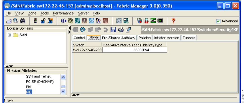
Figure 10-12 IKE Global Tab Information
