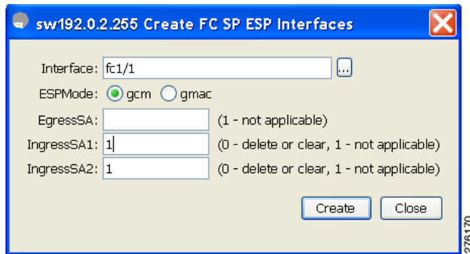
Figure 15-9 Create ESP Interfaces
