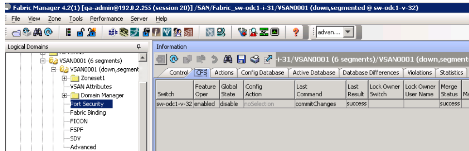
Figure 12-6 Port Security CFS
