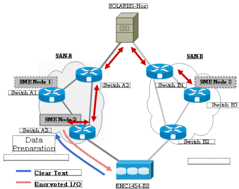
Figure 6-2 SME Disk Offline Data Preparation Architecture
