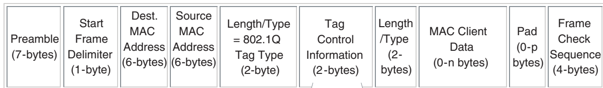
Figure 3-3 Header With 802.1Q Tag
