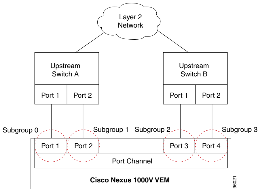
Figure 5-3 Using MAC Pinning to Connect a Port Channel to Multiple Upstream Switches
