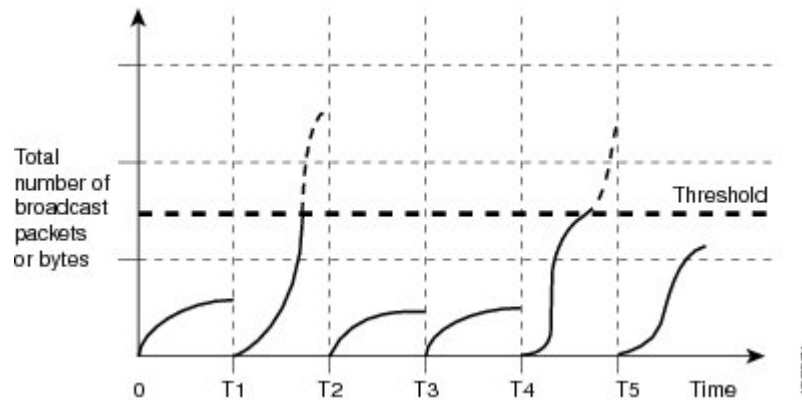
Figure 19: Broadcast Suppression
