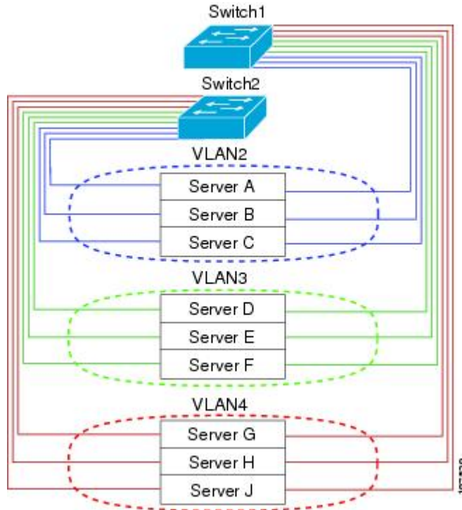
Figure 2: VLANs as Logically Defined Networks
