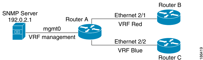
Figure 12-5 Service VRF Reachability Filtering
