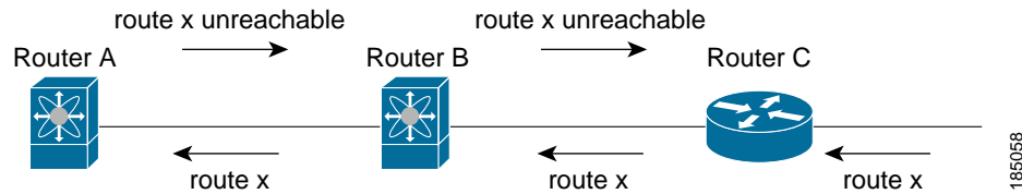
Figure 12-1 RIP with Split Horizon Poison Reverse
