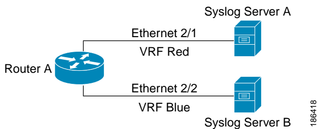
Figure 9-3 Service VRF Filtering
