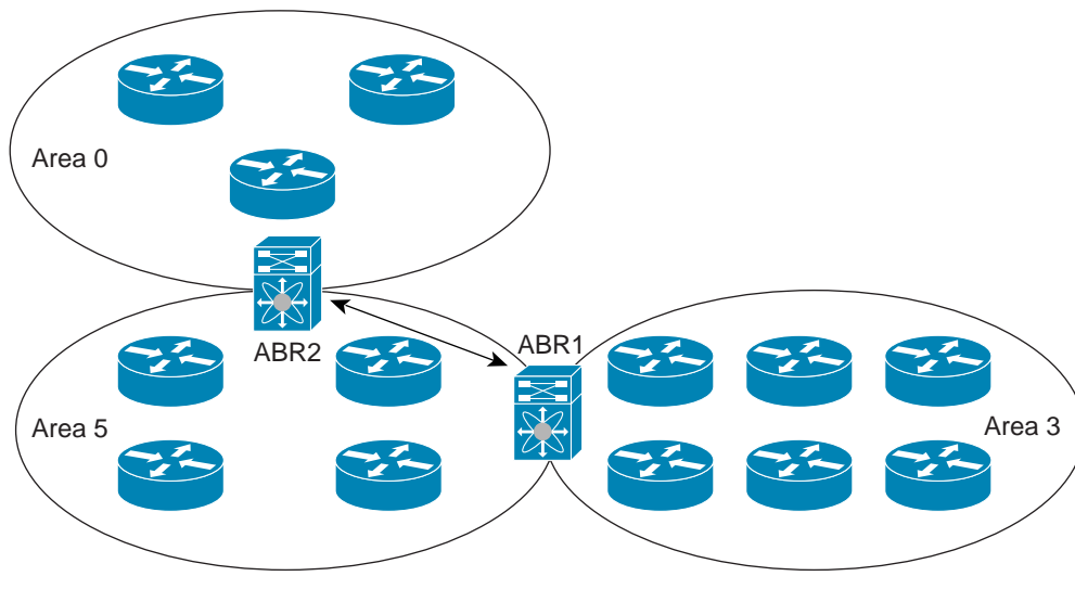
Figure 3-4 Virtual Links
