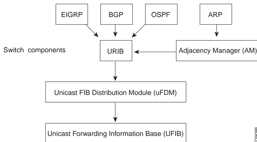
Figure 10-1 Cisco NX-OS Forwarding Architecture
