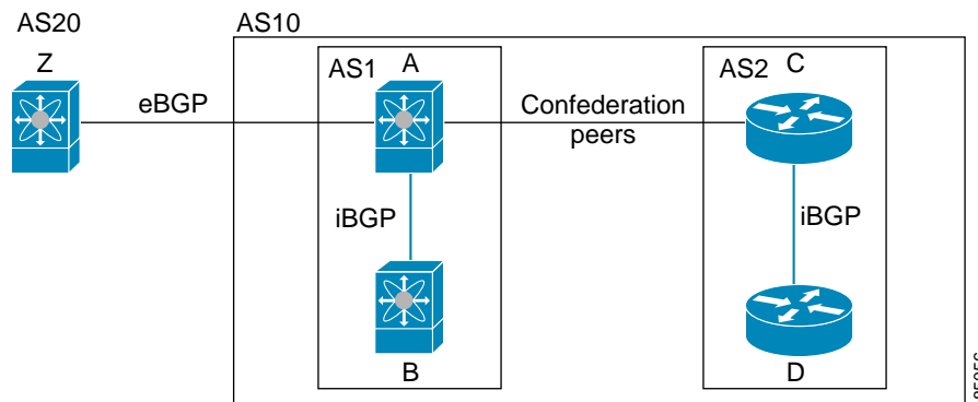
Figure 6-2 AS Confederation
