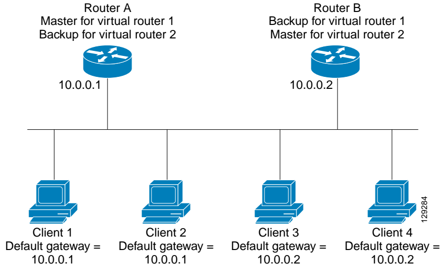
Figure 13-2 Load Sharing and Redundancy VRRP Topology
