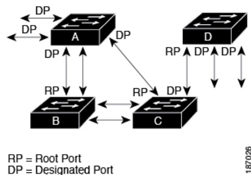
Figure 7: Spanning Tree Topology
