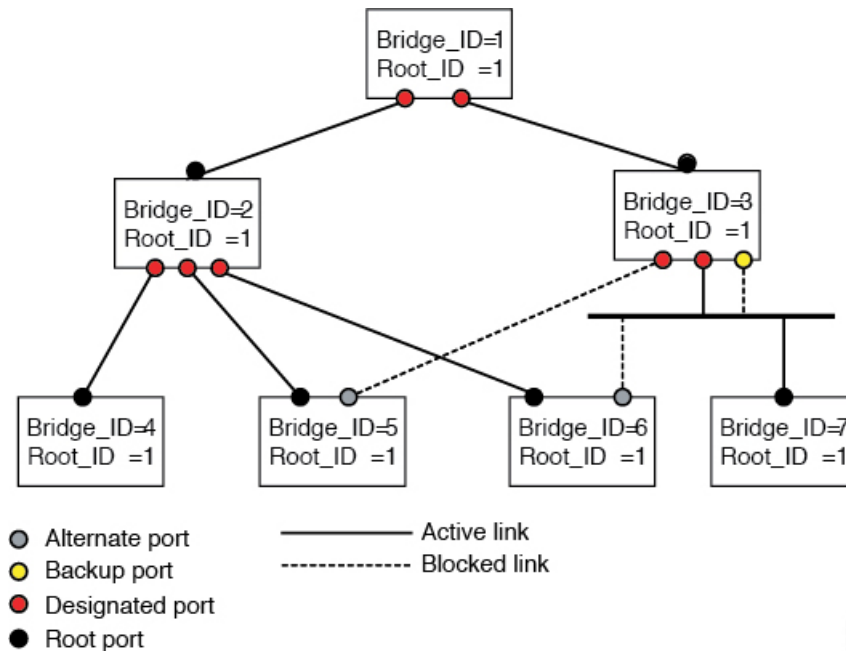
Figure 10: Sample Topology Demonstrating Port Roles
