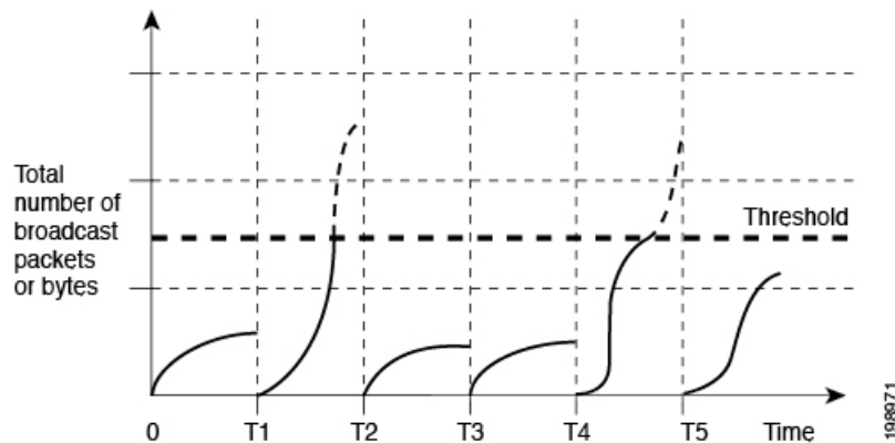
Figure 18: Broadcast Suppression
