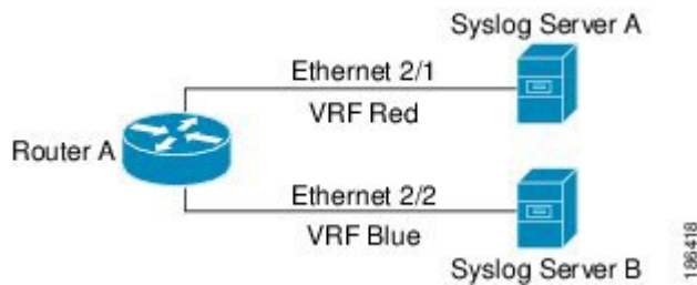
Figure 22: Service VRF Filtering
