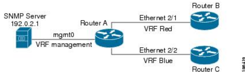
Figure 19: Service VRF Reachability Filtering
