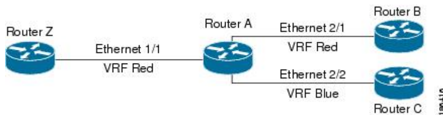
Figure 16: VRFs in a Network
