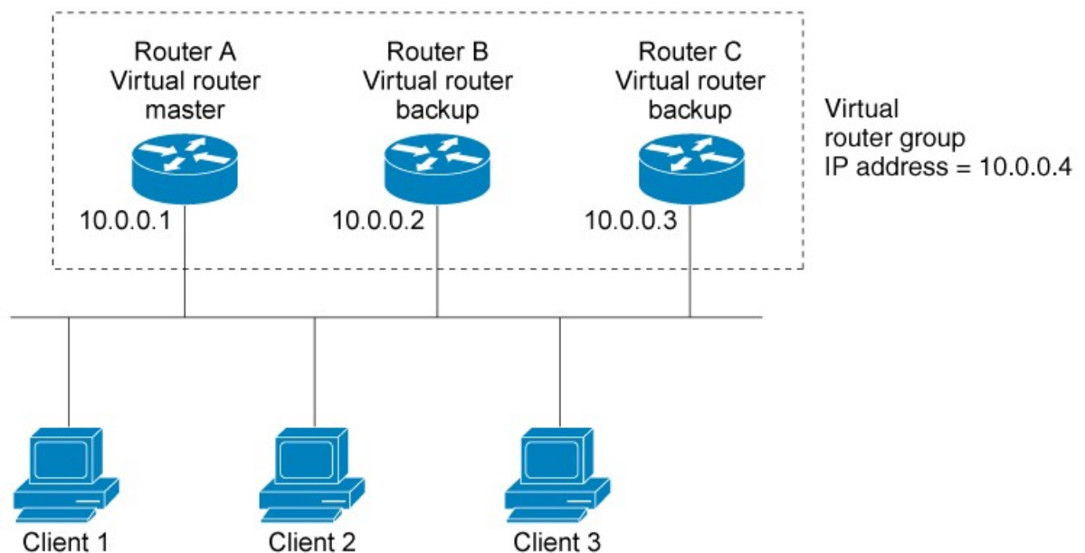
Figure 23: Basic VRRP Topology
