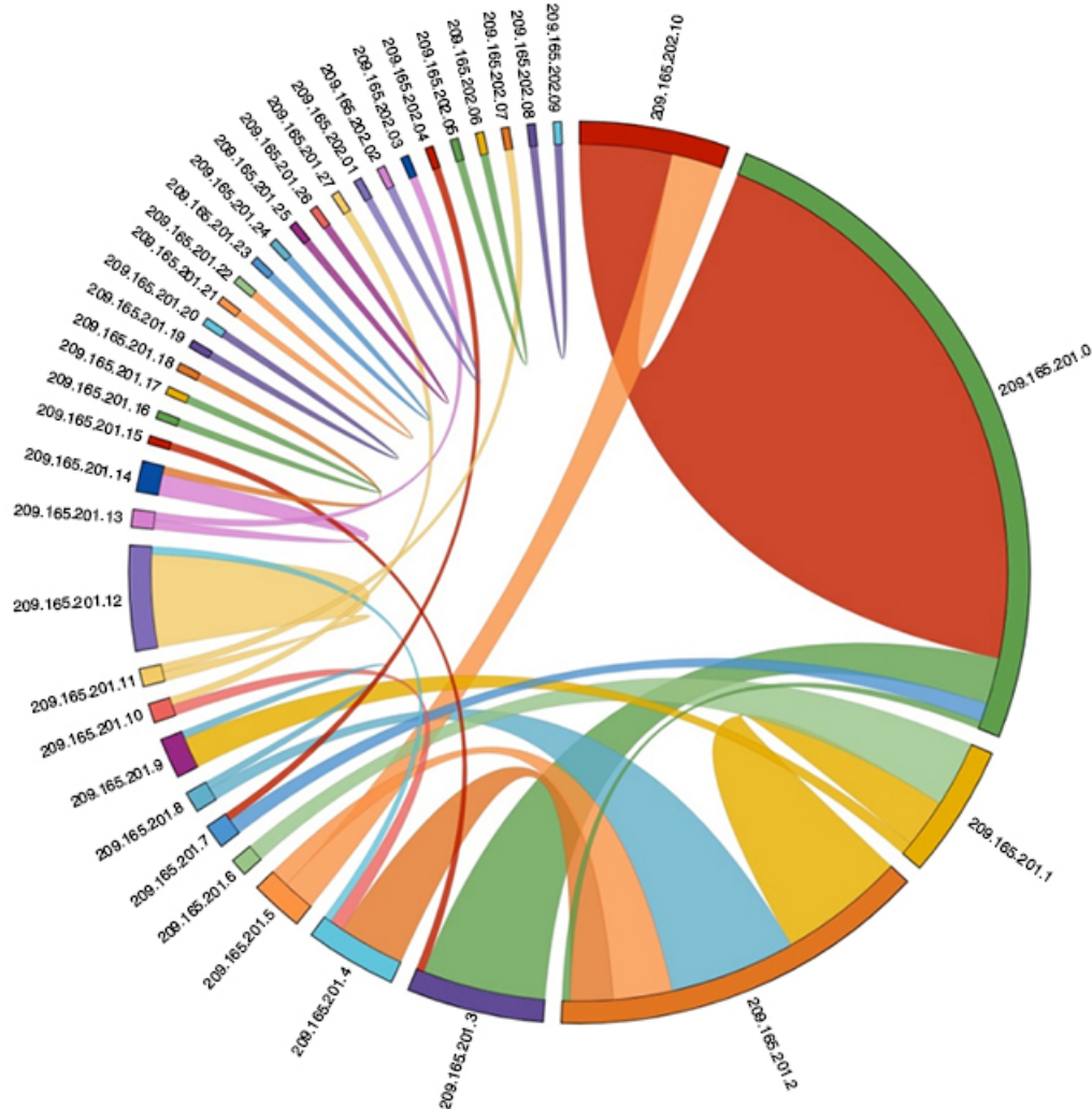
Figure 7: Anomaly Visualization
