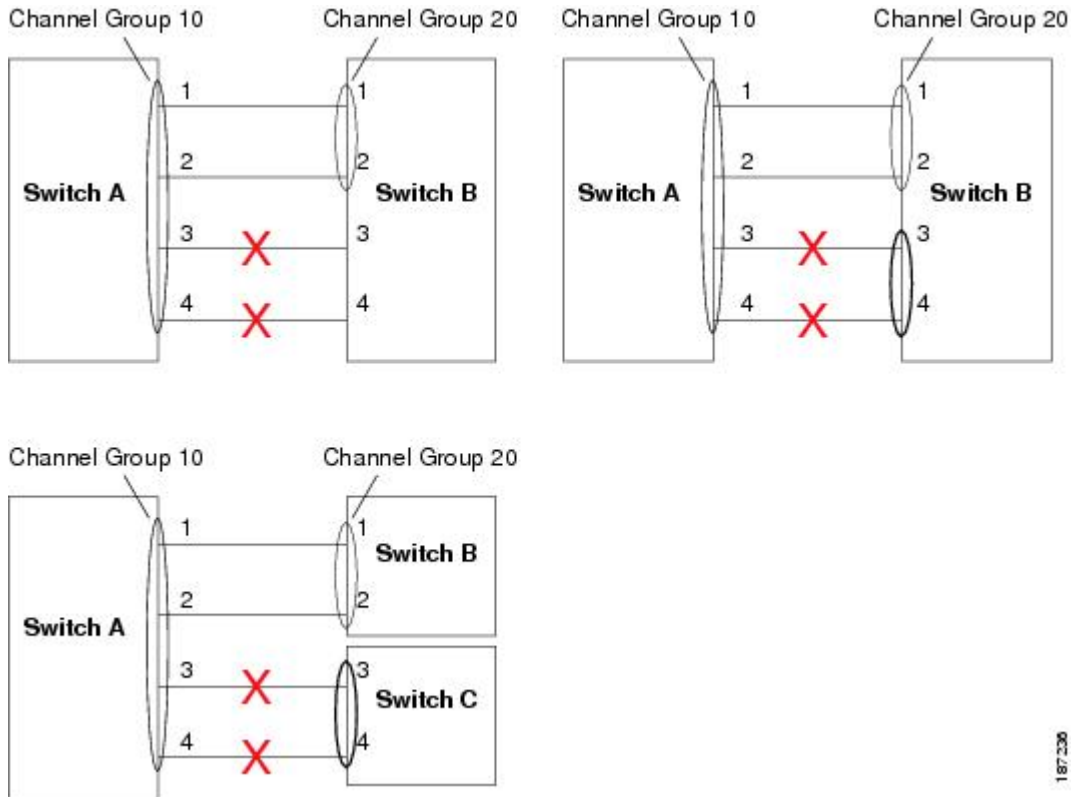
Figure 6: Misconfigured Configurations
