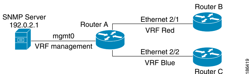
Figure 1-4 Service VRF Reachability Filtering
