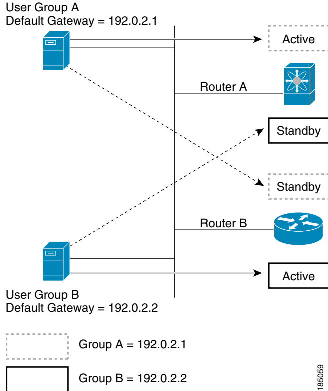
Figure 1-2 HSRP Load Sharing
