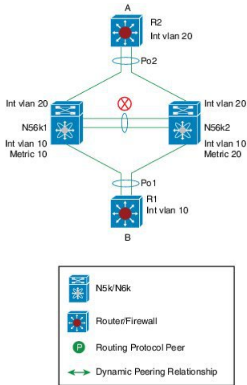
Figure 22: Peering Across vPC Interfaces with Unequal L3 metrics
