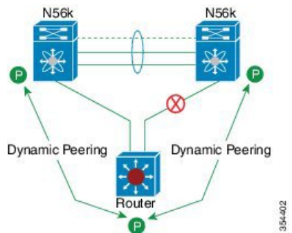
Figure 15: Peering Established Over an STP Interconnection Using a vPC VLAN.
