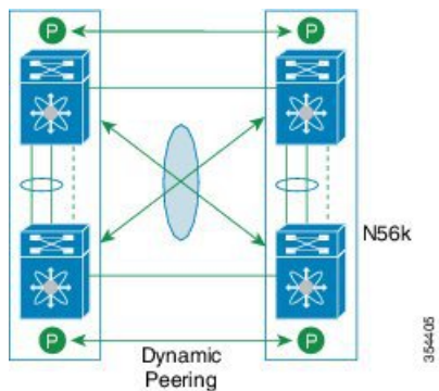
Figure 18: Peering Over a vPC Interconnection (DCI Case)
