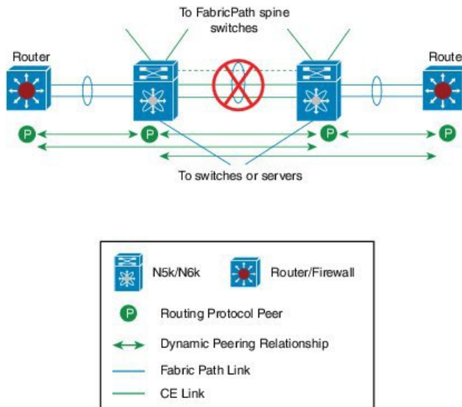
Figure 25: Peering over PC Interconnection and Over vPC+ Peer Link Using vPC VLAN
