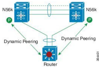
Figure 15: Peering Established Over an STP Interconnection Using a vPC VLAN.
