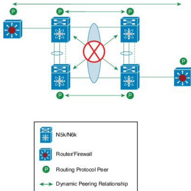
Figure 20: Orphan Device Peering over vPC Interconnection (DCI Case)
