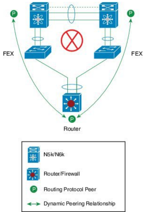
Figure 22: Peering Across vPC Interfaces with Unequal L3 metrics
