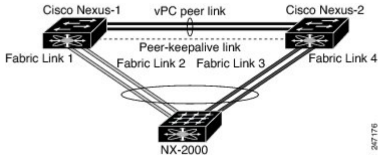
Figure 26: vPC Configuration Example
