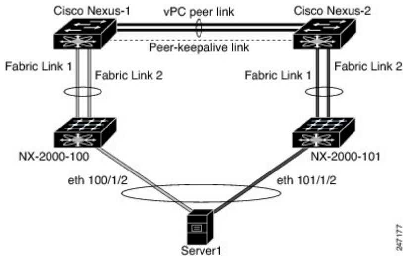
Figure 27: vPC Configuration Example
