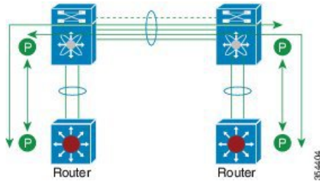
Figure 17: Peering over PC Interconnection and Over vPC peer Link Using vPC VLAN.
