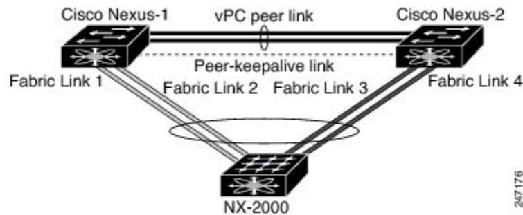
Figure 12: Dual Homed Fabric Extender vPC Topology
