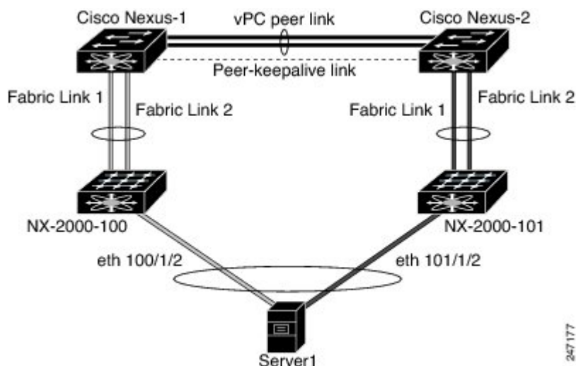
Figure 11: Single Homed Fabric Extender vPC Topology
