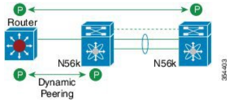
Figure 17: Peering over PC Interconnection and Over vPC peer Link Using vPC VLAN.
