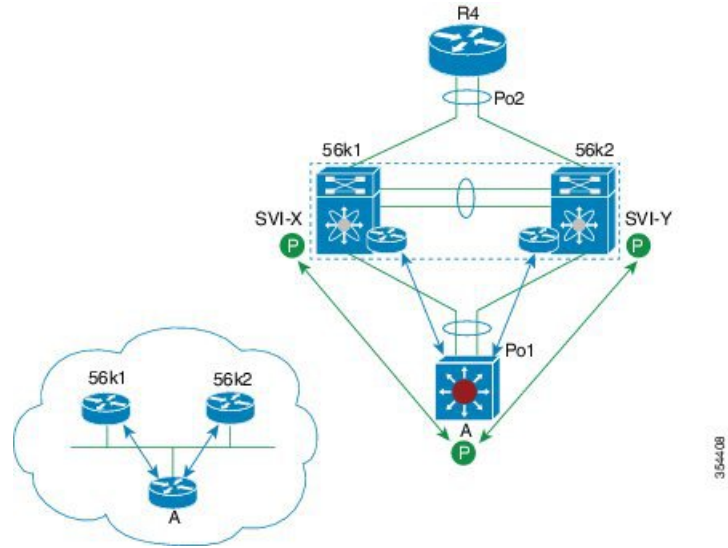
Figure 13: Layer 3 over vPC Solution
