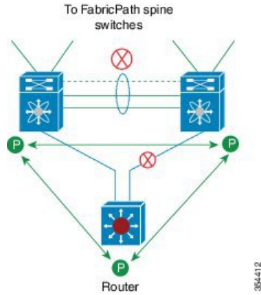
Figure 24: Route Peering with Orphan Device with Both the vPC+ peers
