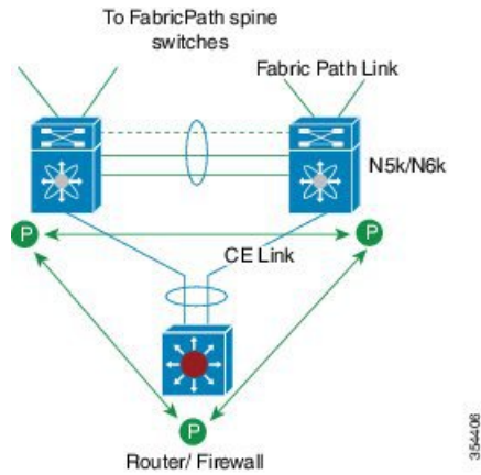
Figure 19: Peering with vPC+
