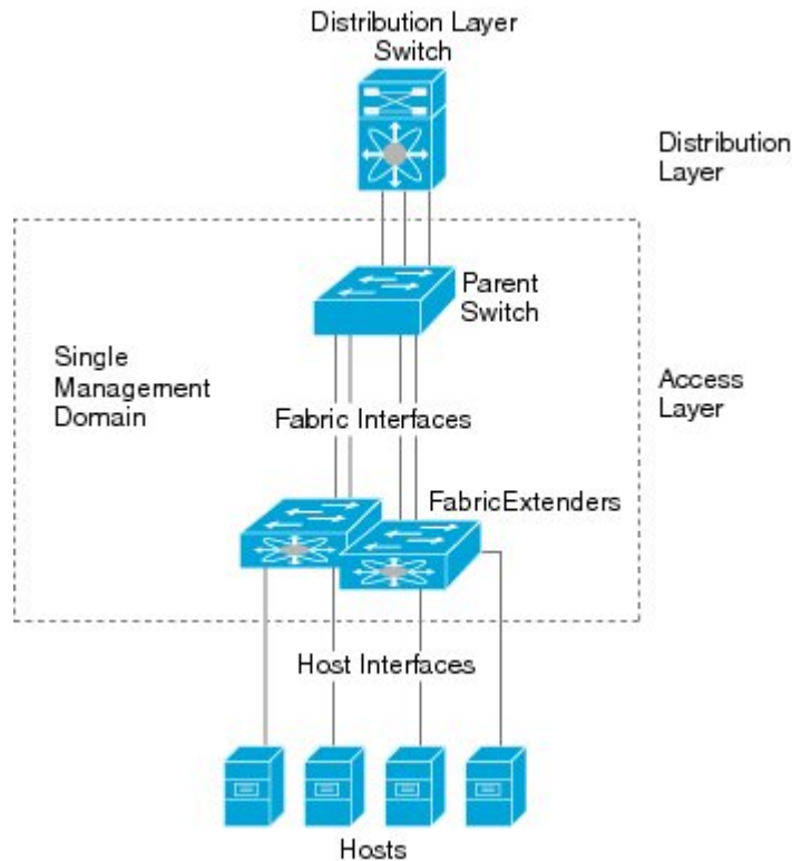
Figure 18: Single Management Domain
