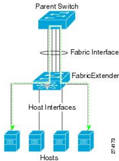
Figure 21: Forwarding Model
