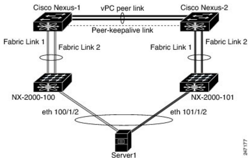
Figure 19: Single Homed Fabric Extender vPC Topology
