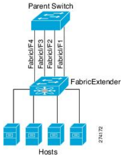
Figure 22: Static Pinning Fabric Interface Connections
