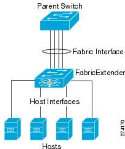
Figure 23: Port Channel Fabric Interface Connection
