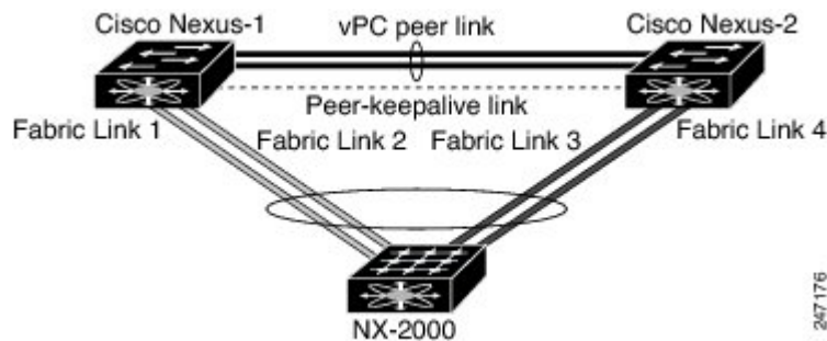
Figure 20: Dual Homed Fabric Extender vPC Topology
