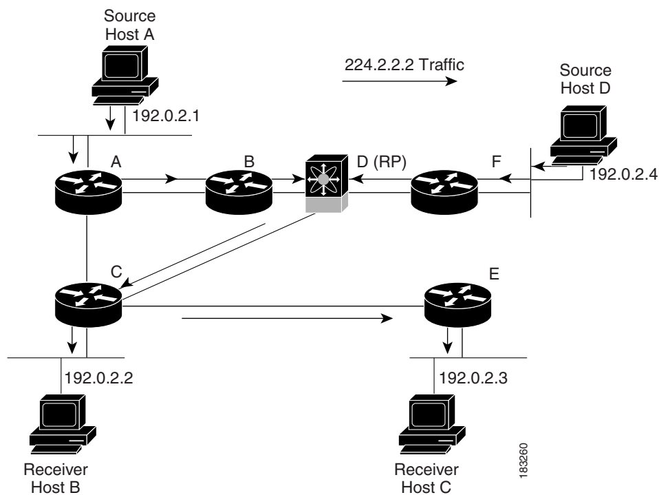
Figure 1-3 Shared Tree
