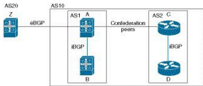
Figure 2: AS Confederation
