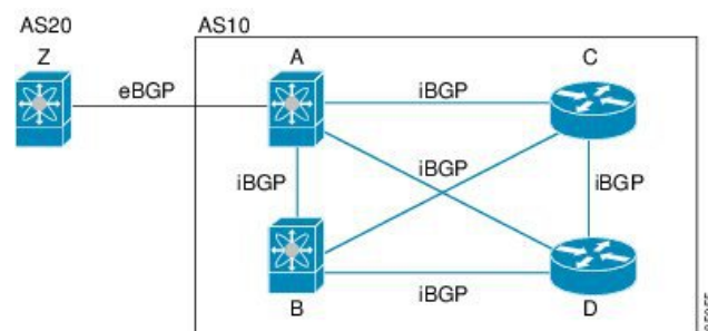
Figure 1: iBGP Network
