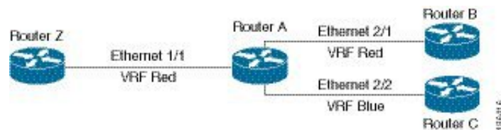
Figure 2: VRFs in a Network
