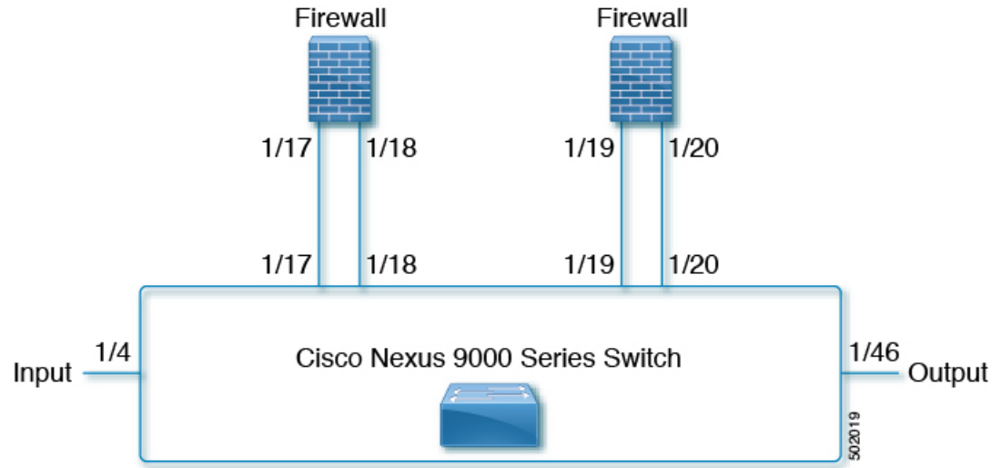
Figure 7: Layer 2 Reverse Configuration
