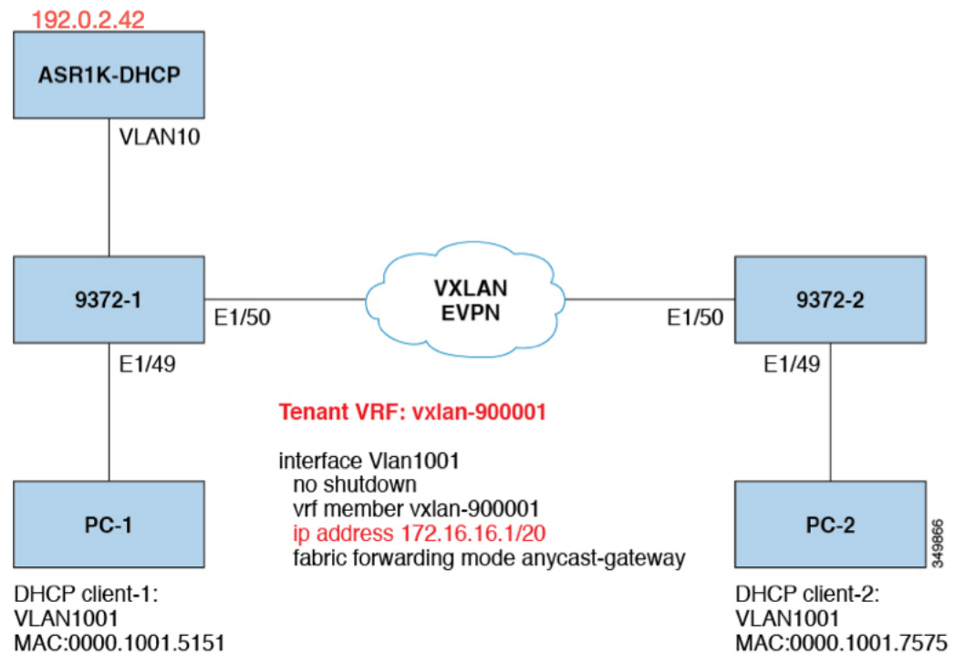
Figure 33: Example Topology
