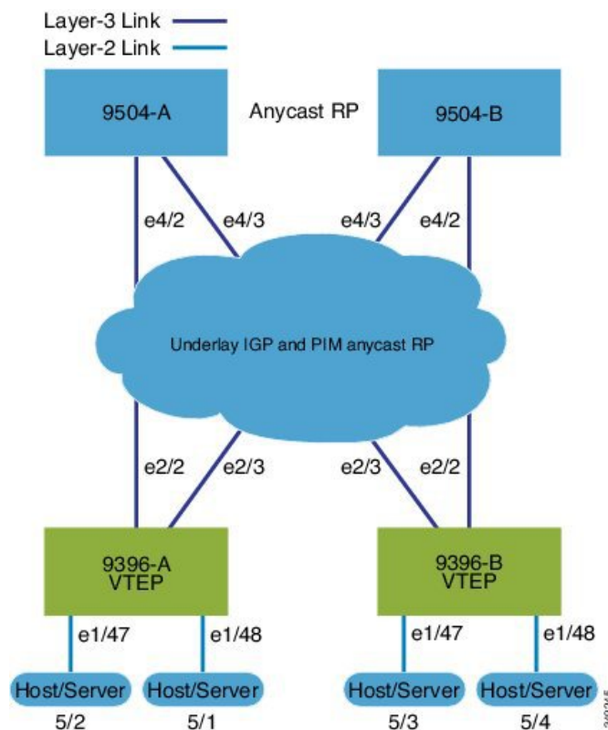
Figure 11: VXLAN BGP EVPN Topology (EBGP)
