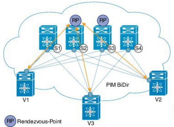
Figure 9: PIM BiDir as the IP multicast routing protocol
