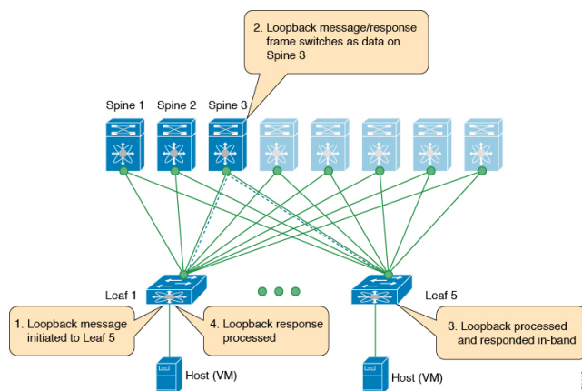
Figure 16: Loopback Message
