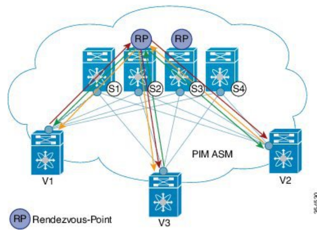
Figure 8: PIM ASM as the IP multicast routing protocol
