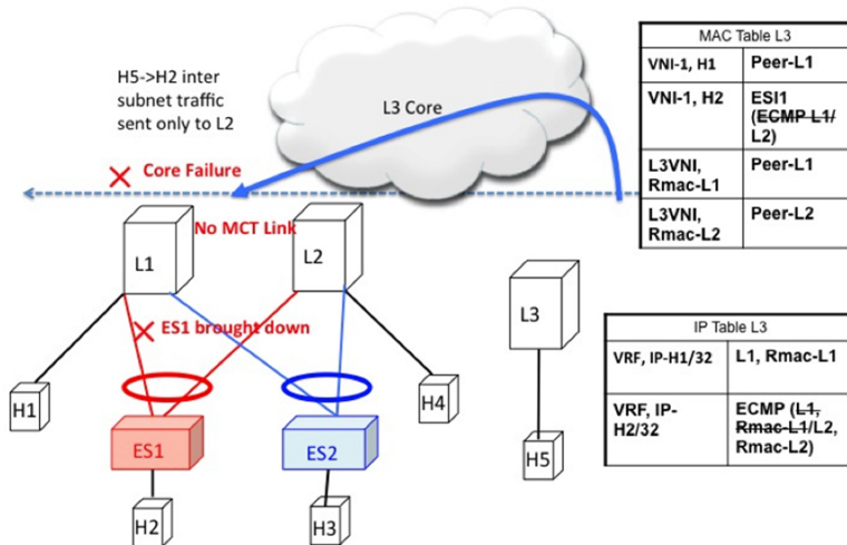
Figure 51: Layer 3 VXLAN Gateway. Core failure. All L3 ECMP paths to L1 are withdrawn at L3 due to route reachability going away.
