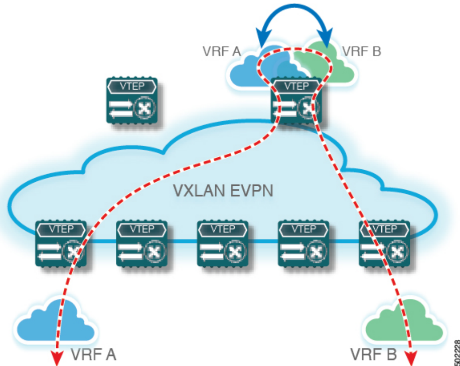
Figure 13: Centralized VRF Route-Leaking - Specific Prefixes with Custom VRF
