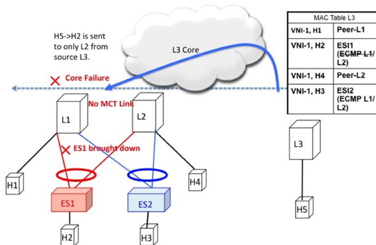
Figure 48: Layer 2 VXLAN Gateway. Core failure at L1. L3 withdraws L1 from MAC ECMP list. This will happen due to route reachability to L1 going away at L3.
