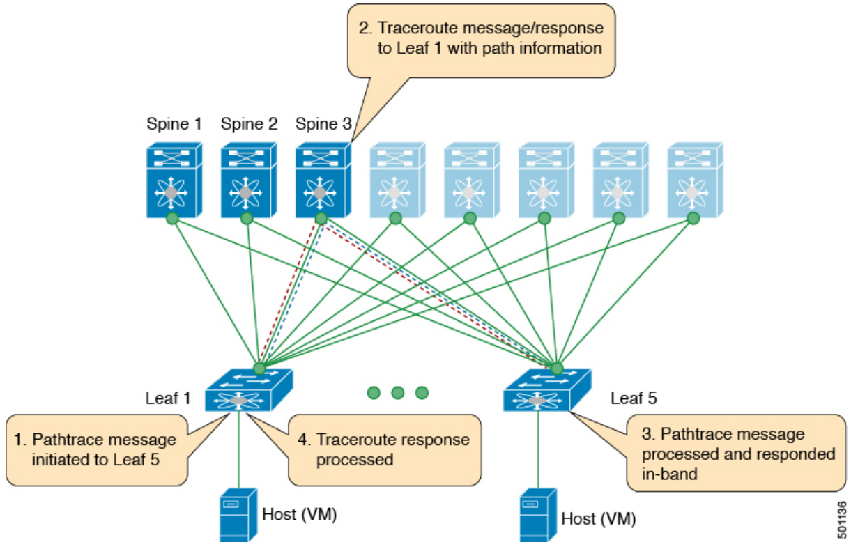
Figure 18: Traceroute Message
