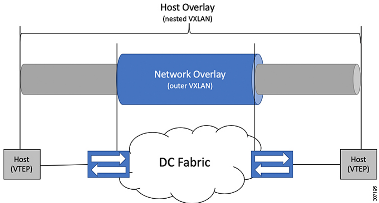
Figure 2: Host Overlay
