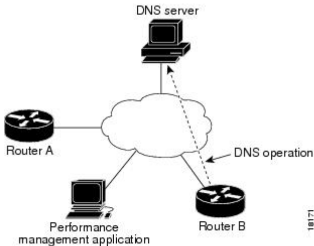
Figure 10: DNS Operation
