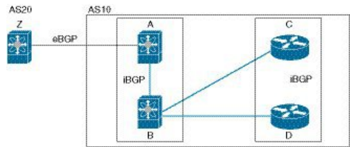
Figure 36: Route Reflector
