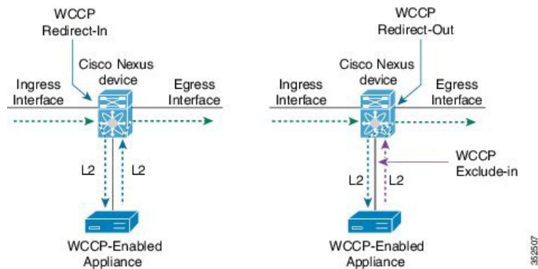
Figure 22: WCCPv2 Redirection
