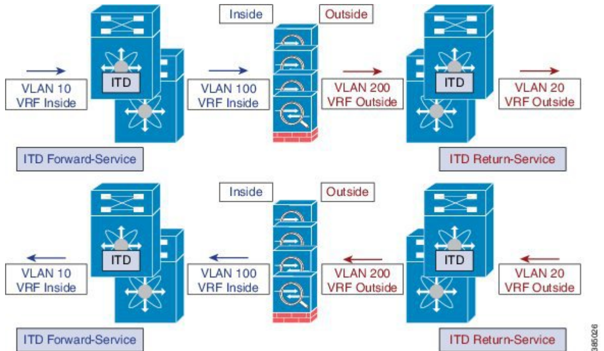
Figure 11: Logical View of the ITD-ASA Deployment
