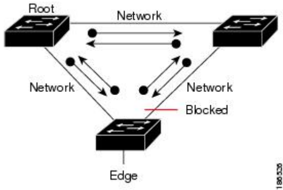
Figure 19: Network STP Topology Running Bridge Assurance
