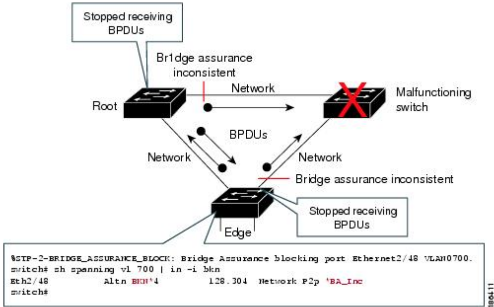
Figure 20: Network Problem Averted with Bridge Assurance Enabled
