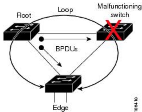
Figure 18: Network Problem without Running Bridge Assurance
