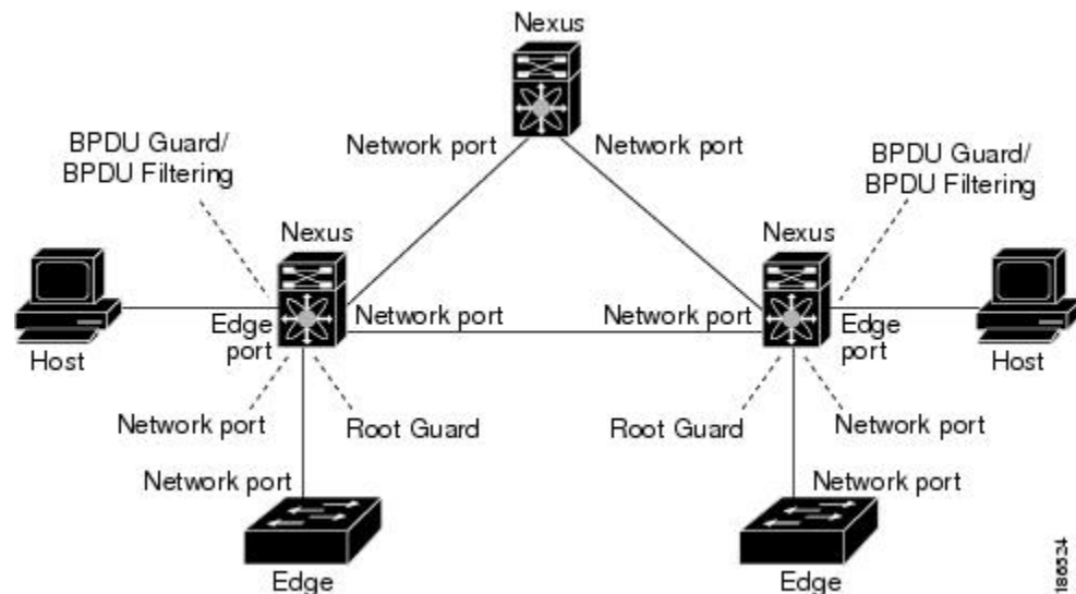
Figure 21: Network with STP Extensions Correctly Deployed
