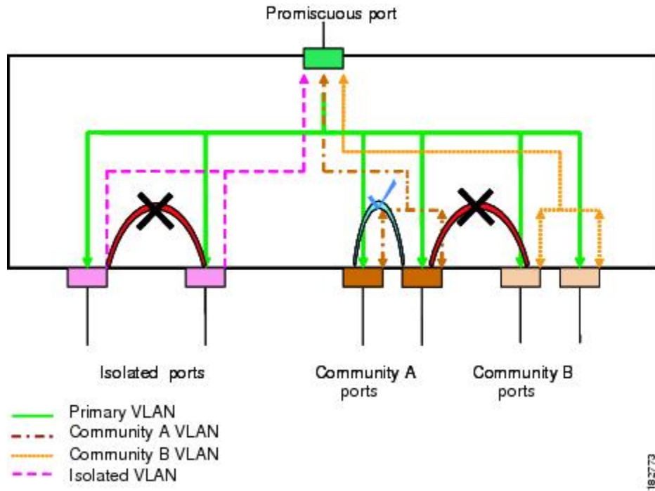
Figure 2: Private VLAN Layer 2 Traffic Flows
