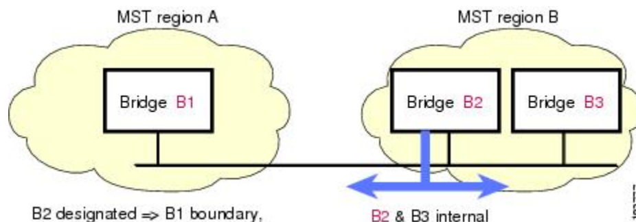
Figure 14: MST Boundary Ports
