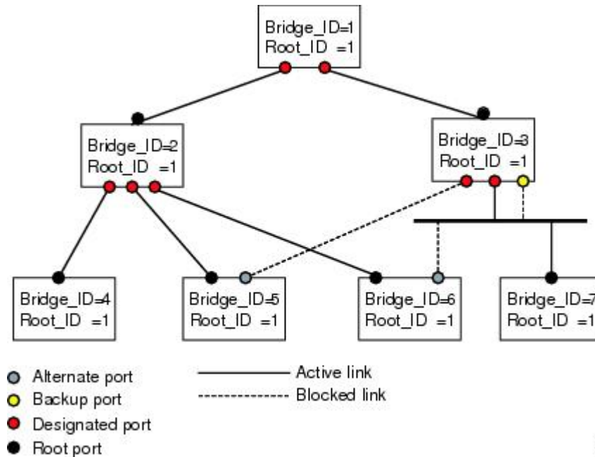
Figure 8: Sample Topology Demonstrating Port Roles
