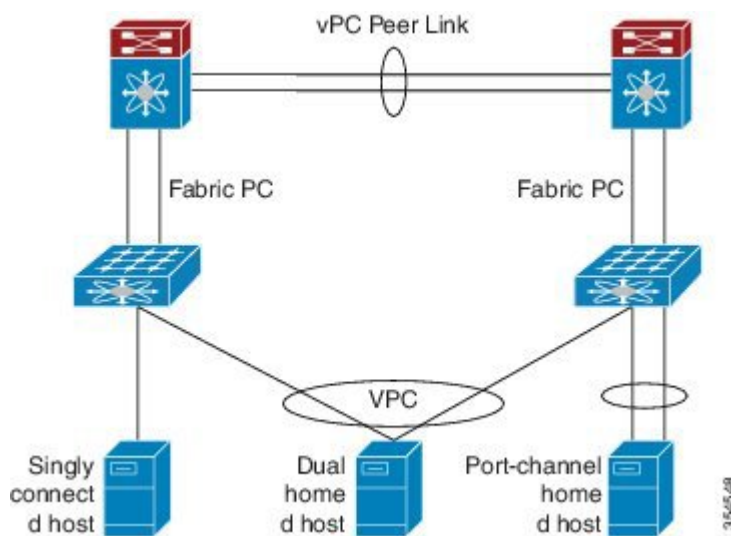
Figure 3: Supported Topology for Isolated PVLAN on FEX HIF
