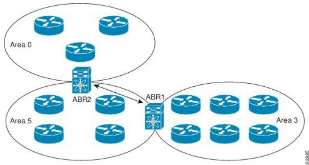
Figure 26: Virtual Links
