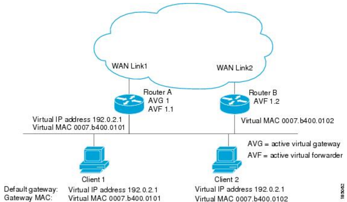
Figure 45: GLBP Topology
