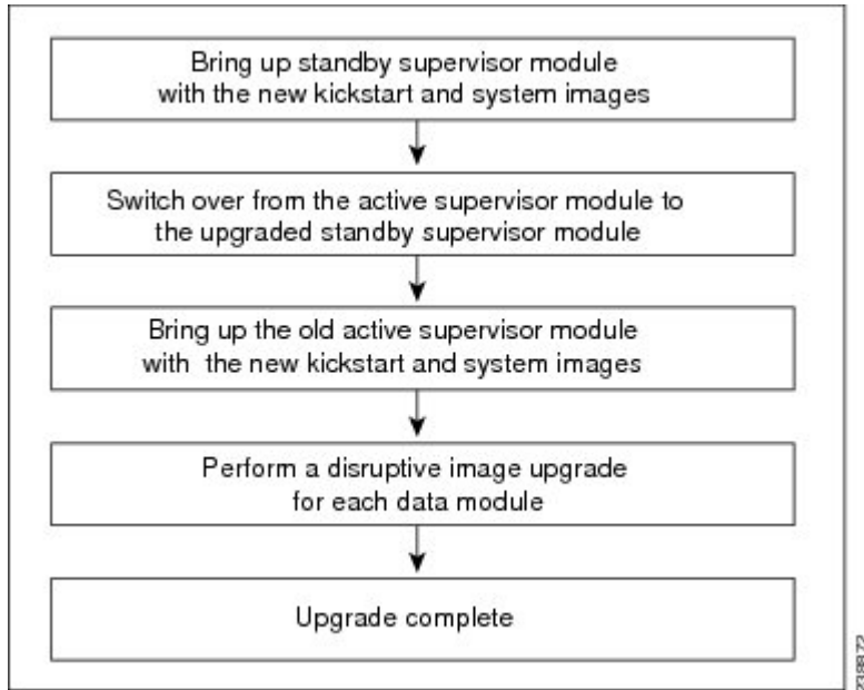
Figure 8: ISSU Process
