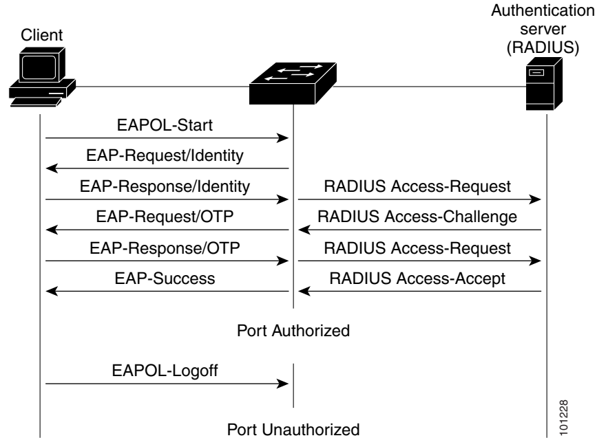
Figure 12-3 Message Exchange
