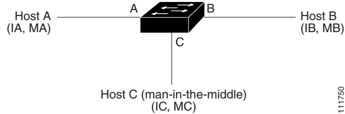
Figure 22-1 ARP Cache Poisoning
