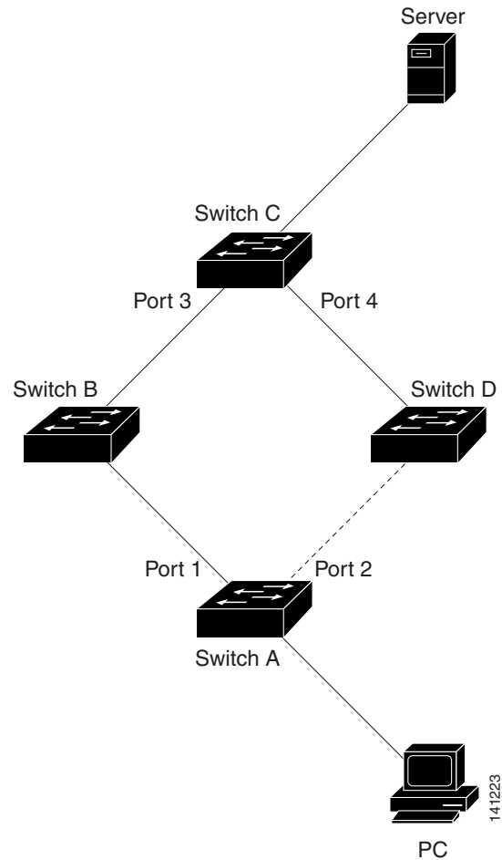
Figure 20-3 MAC Address-Table Move Update Example
