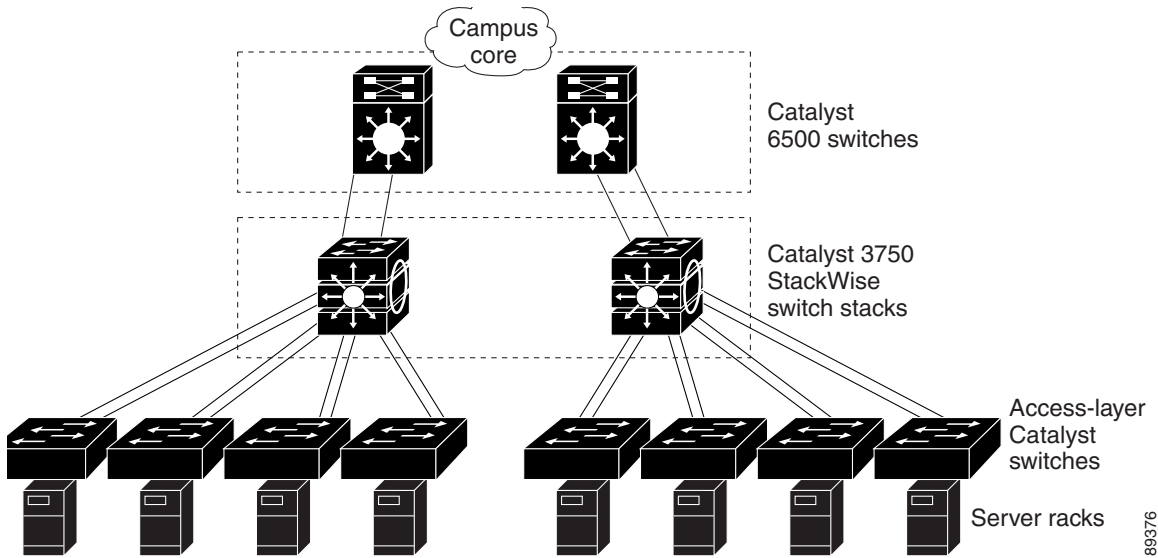
Figure 1-3 Server Aggregation
