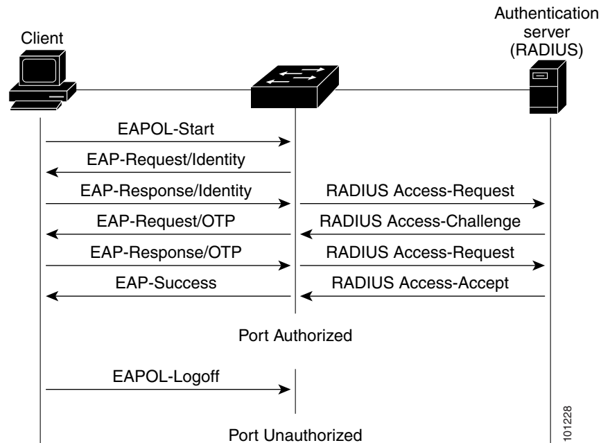
Figure 12-3 Message Exchange
