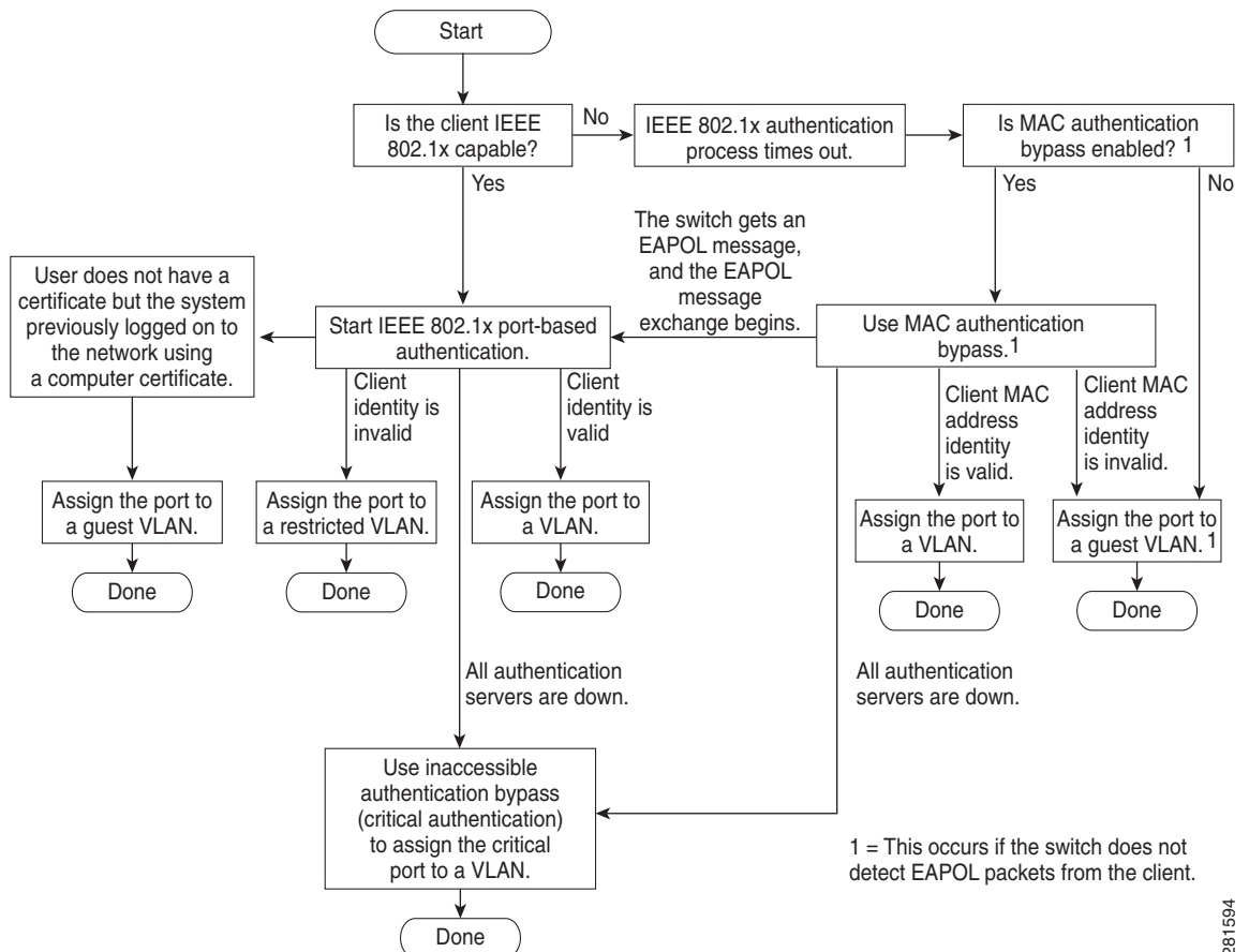
Figure 12-2 Authentication Flowchart
