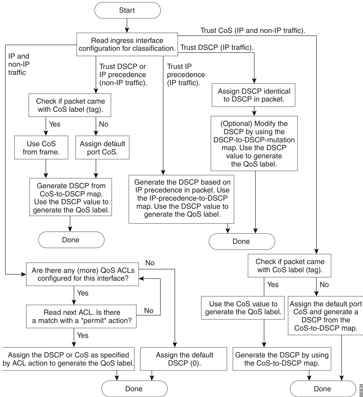
Figure 34-3 Classification Flowchart
