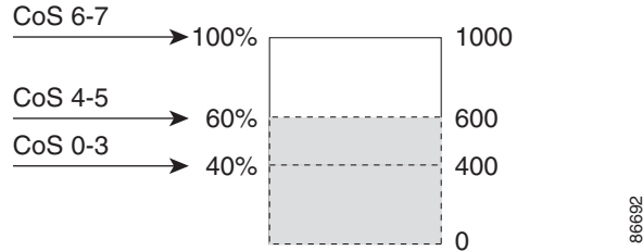
Figure 34-6 WTD and Queue Operation
