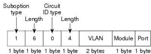
Figure 62: Suboption Packet Formats
