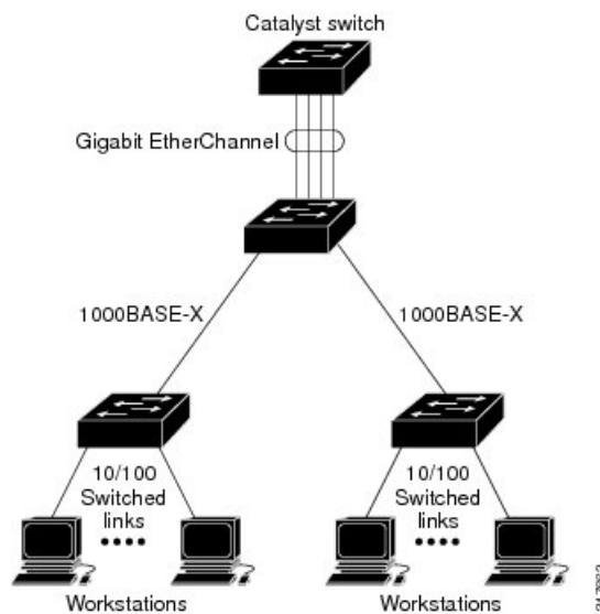
Figure 90: Typical EtherChannel Configuration
