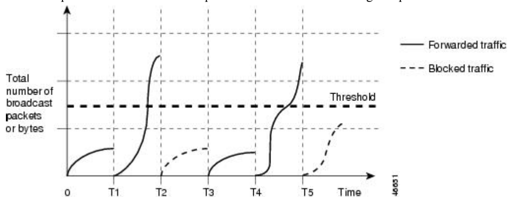
Figure 66: Broadcast Storm Control Example
