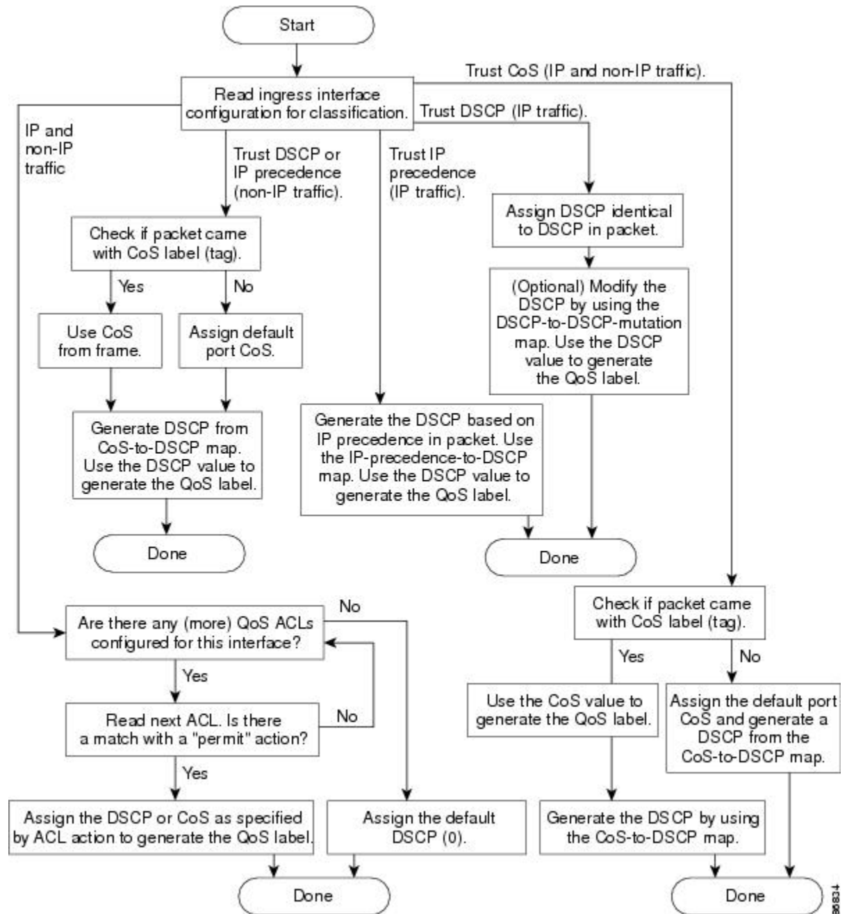
Figure 80: Classification Flowchart
