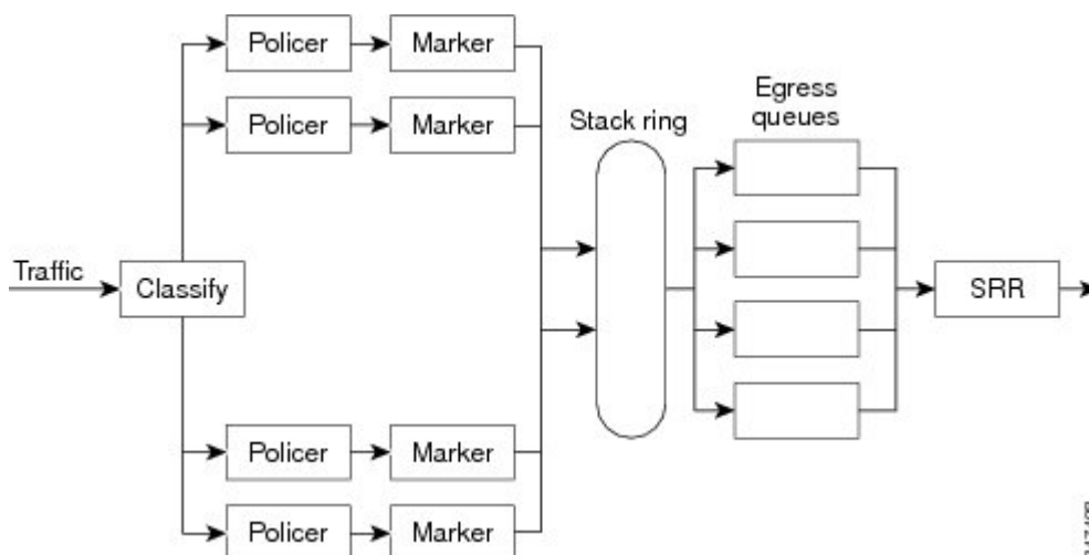
Figure 82: Ingress and Egress Queue Location on Switch
