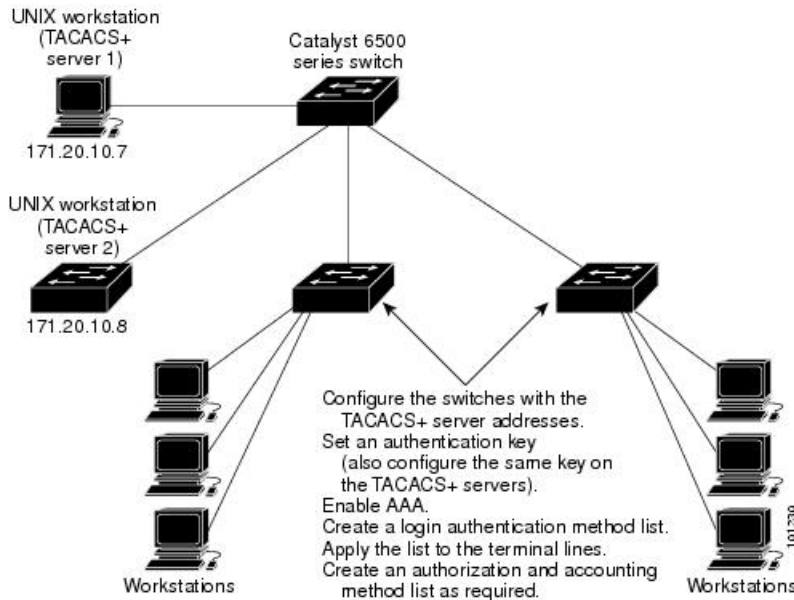
Figure 21: Typical TACACS+ Network Configuration
