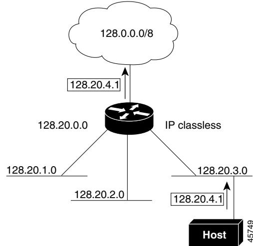
Figure 33-2 IP Classless Routing
