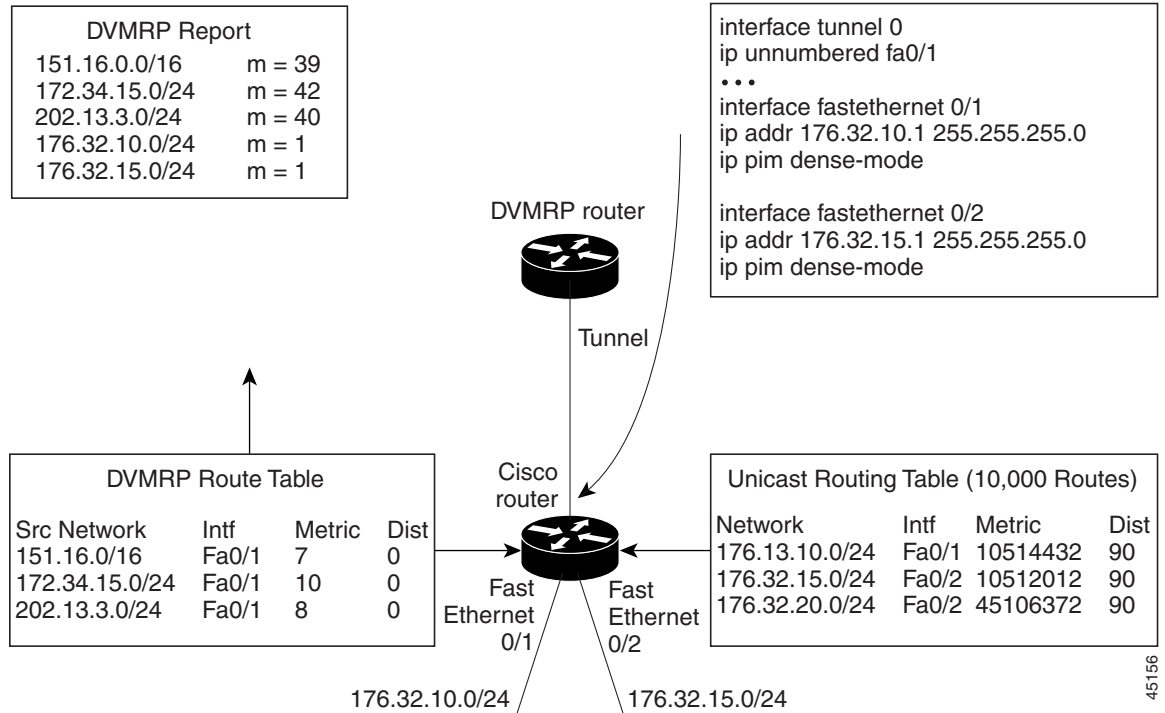
Figure 43-10 Only Connected Unicast Routes Are Advertised by Default
