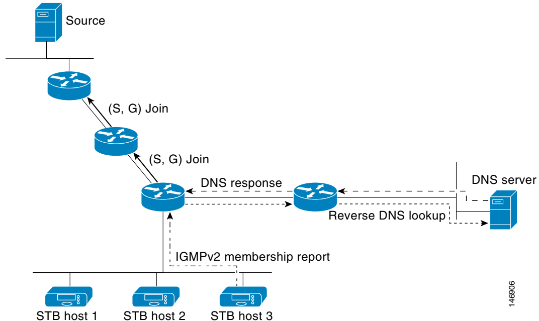
Figure 43-4 DNS-Based SSM-Mapping
