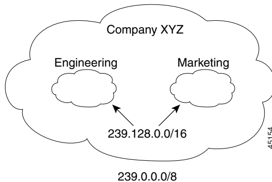
Figure 43-7 Administratively-Scoped Boundaries
