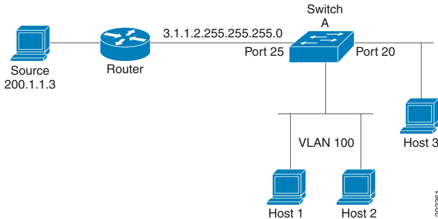
Figure 43-2 PIM Stub Router Configuration
