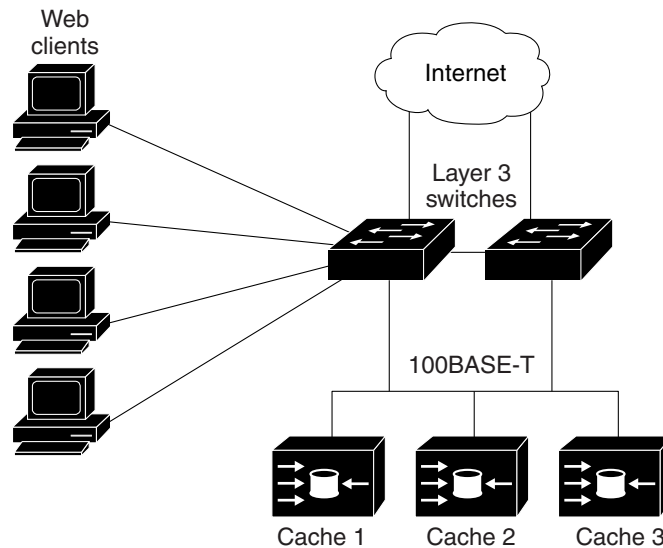
Figure 44-1 Cisco Cache Engine and WCCP Network Configuration
