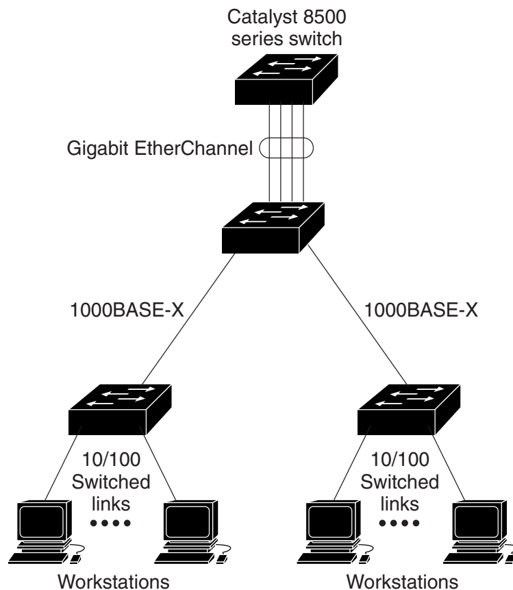
Figure 35-1 Typical EtherChannel Configuration
