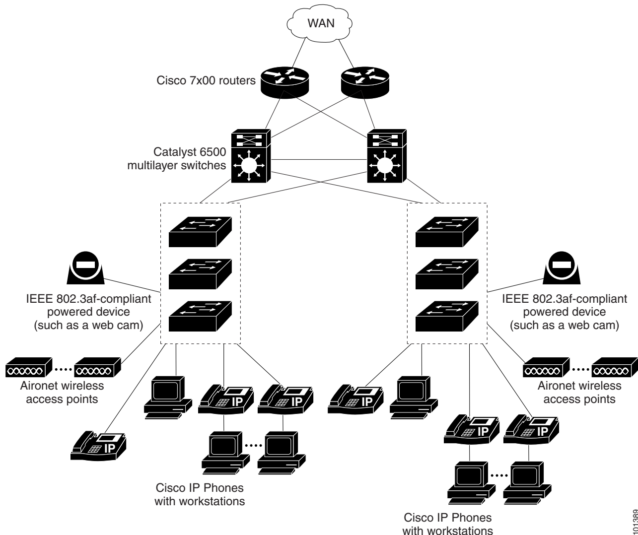
Figure 1-5 Switches in Wiring Closets in a Backbone Configuration
