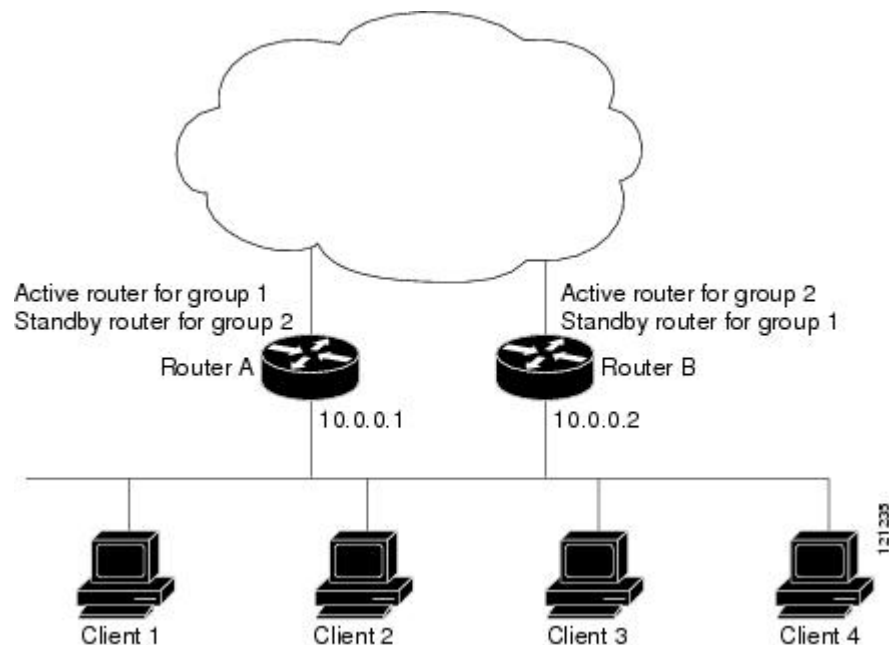
Figure 2: MSHRP Load Sharing
