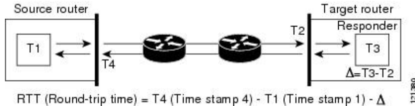
Figure 6: Cisco IOS IP SLA Responder Time Stamping
