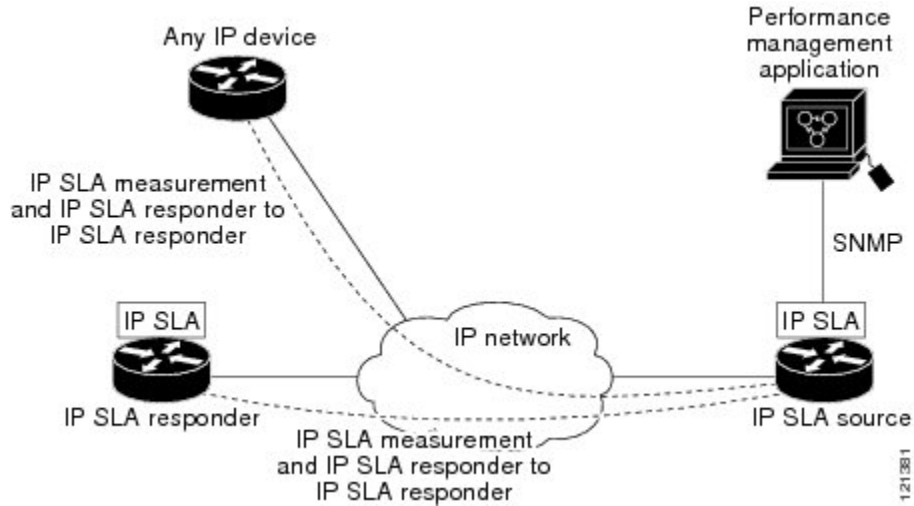
Figure 5: Cisco IOS IP SLAs Operation
