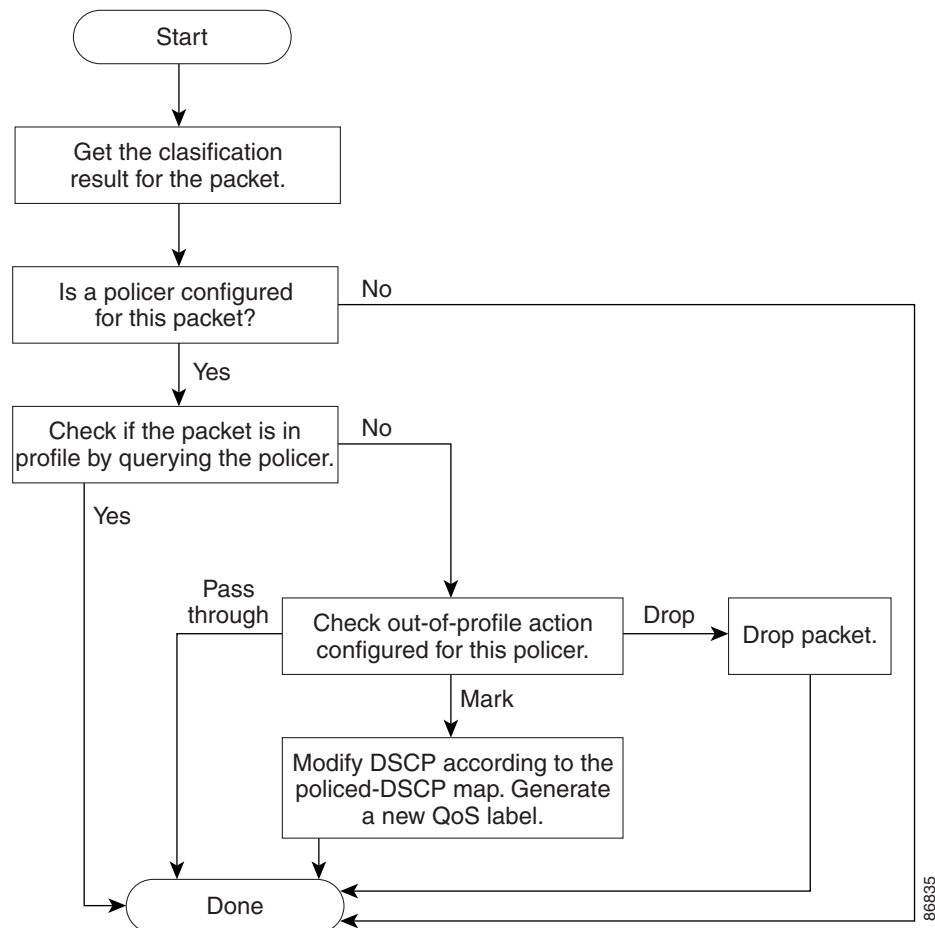
Figure 32-4 Policing and Marking Flowchart
