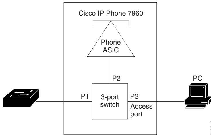
Figure 16-1 Cisco 7960 IP Phone Connected to a Switch
