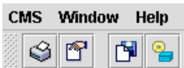
Figure 3-1 Menu Bar
