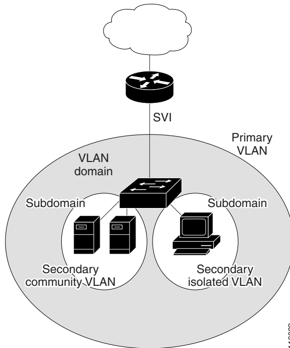
Figure 15-1 Private-VLAN Domain
