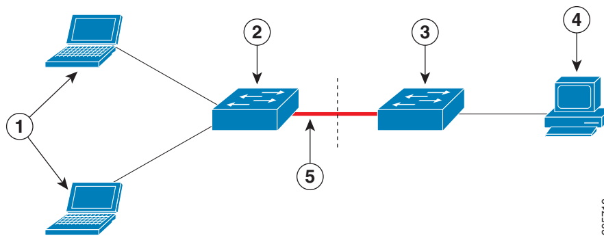
Figure 11-6 Authenticator and Supplicant Switch using CISP
