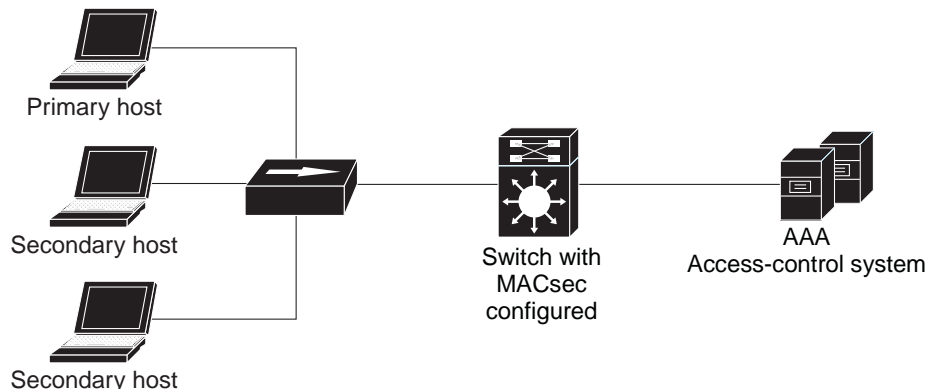
Figure 11-8 MACsec in Standard Multiple-Host Mode - Unsecured
