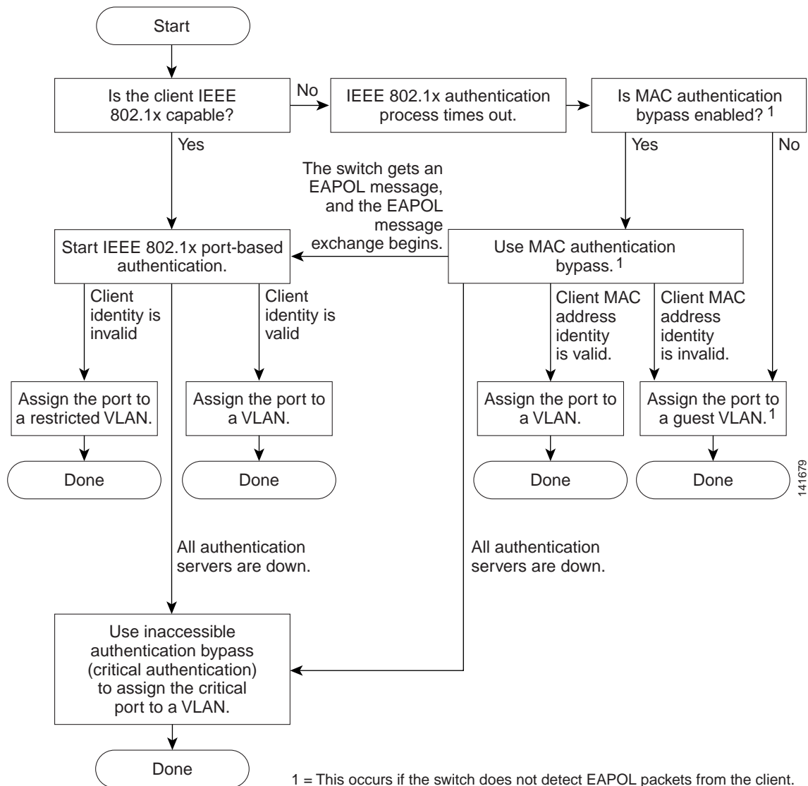
Figure 11-2 Authentication Flowchart
