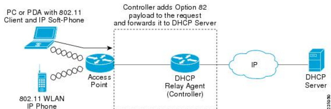
Figure 127: DHCP Option 82
