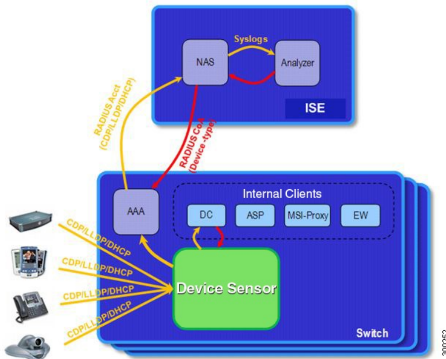
Figure 111: Device Sensor Clients
