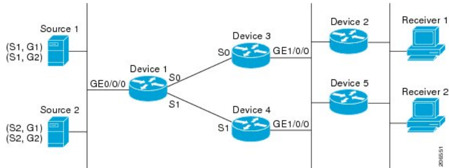
Figure 35: ECMP Multicast Load Splitting and the PIM Assert Process in PIM-SM and PIM-SSM
