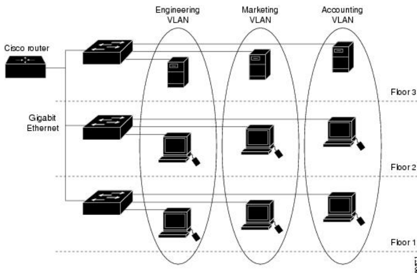
Figure 124: VLANs as Logically Defined Networks
