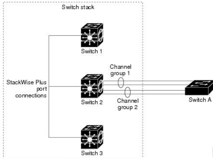
Figure 56: Single-Switch EtherChannel
