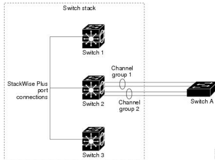
Figure 57: Single-Switch EtherChannel
