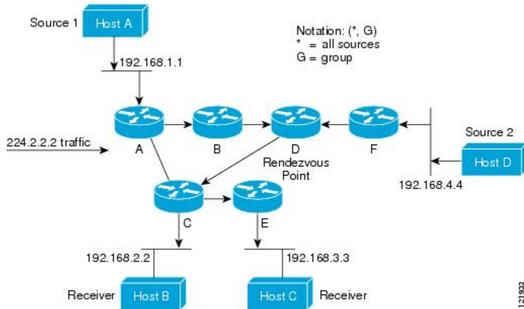
Figure 22: Shared Tree
