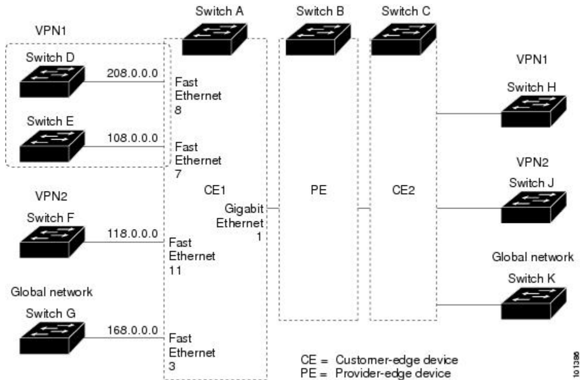
Figure 95: Multi-VRF CE Configuration Example
