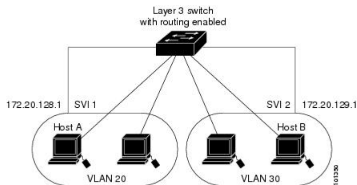
Figure 2: Connecting VLANs with the Switch
