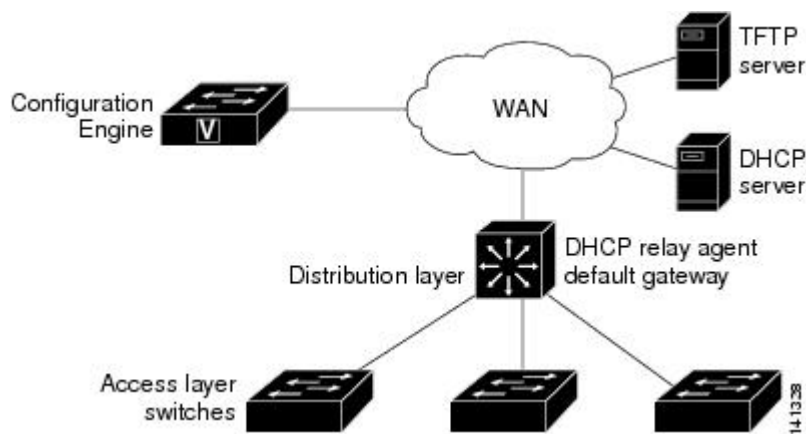
Figure 71: Initial Configuration
