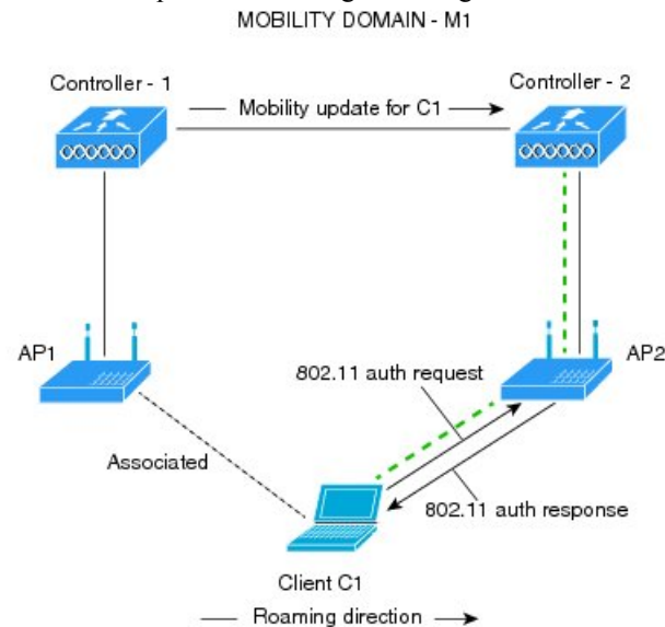
Figure 136: Message Exchanges when Over the Air client roaming is configured
