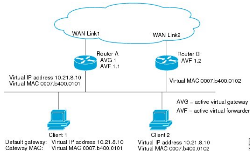
Figure 15: GLBP Topology
