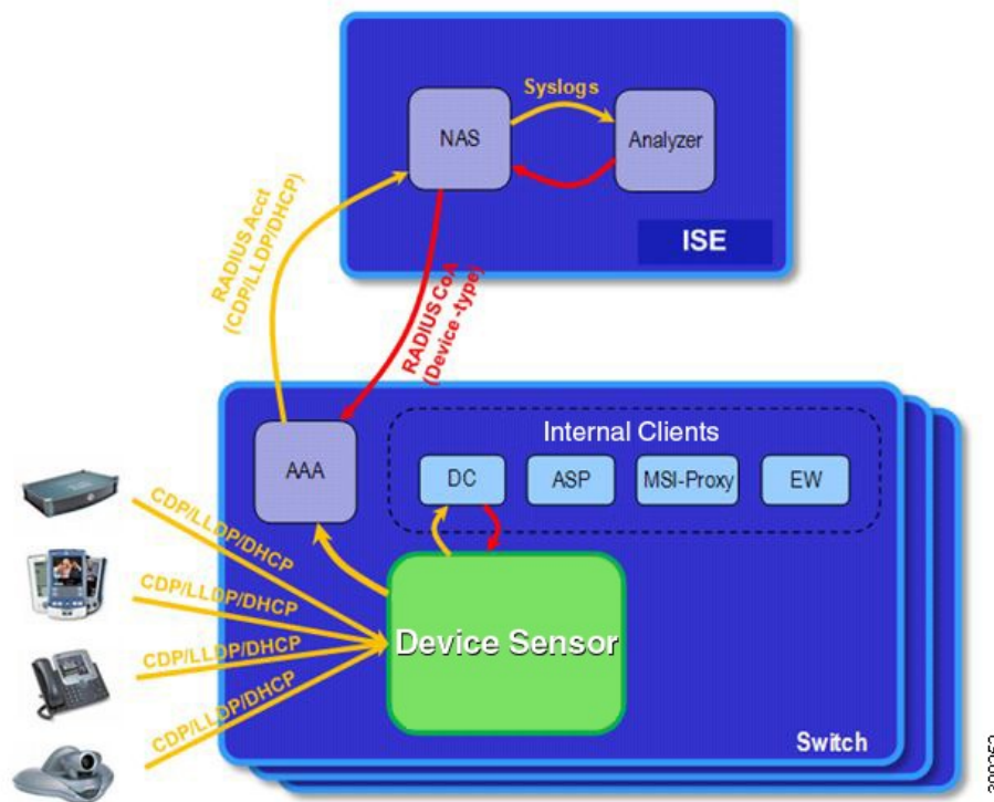
Figure 26: Device Sensor Clients
