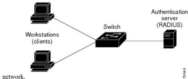
Figure 27: Web-Based Authentication Device Roles
