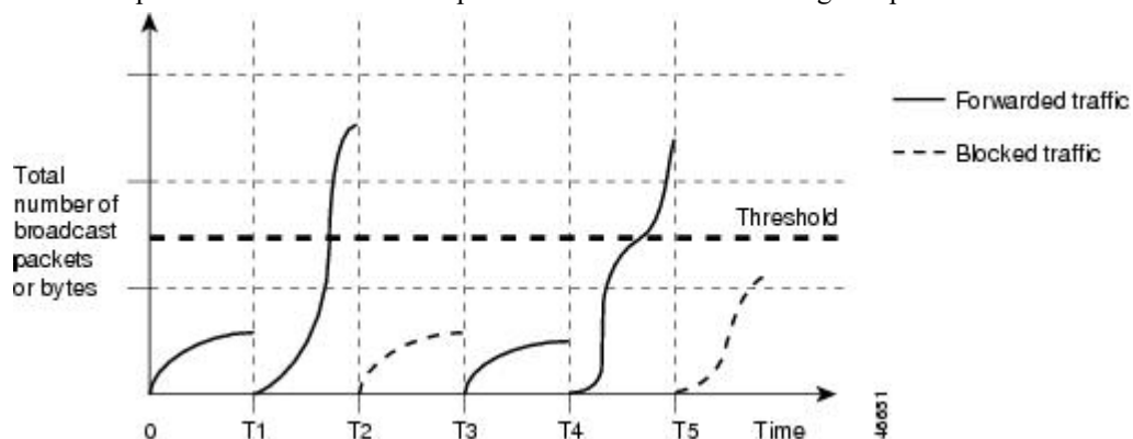
Figure 32: Broadcast Storm Control Example
