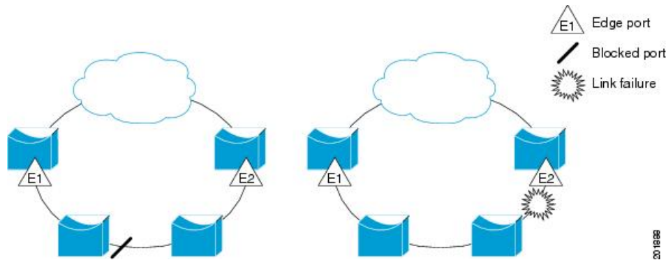
Figure 26: REP Open Segment
