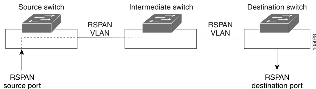
Figure 45-2 Example of RSPAN Configuration
