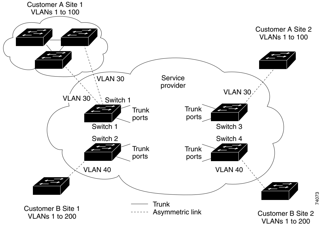
Figure 23-4 Layer 2 Protocol Tunneling
