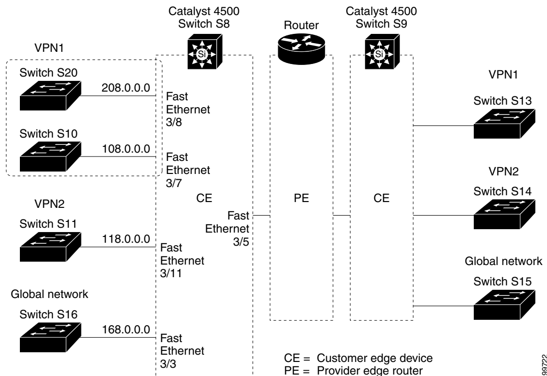
Figure 34-2 VRF-lite Configuration Example
