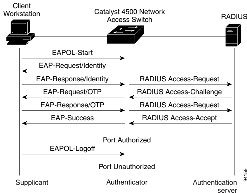
Figure 38-2 Message Exchange
