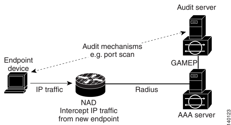
Figure 41-3 NAC Device Roles
