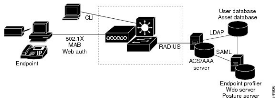
Figure 34: Sample Deployment of Cisco IBNS
