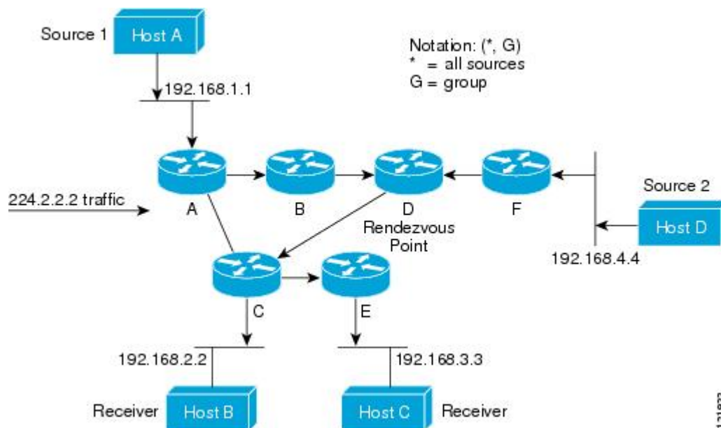
Figure 15: Shared Tree
