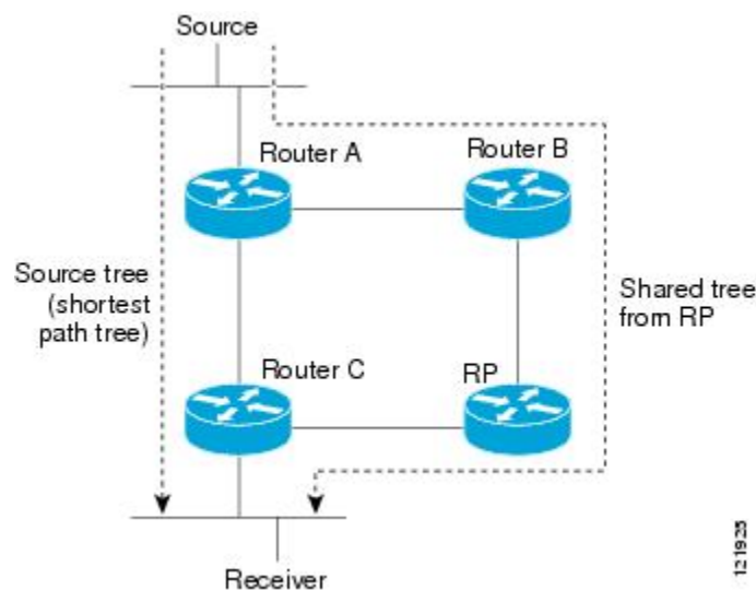
Figure 26: Shared Tree versus Source Tree (Shortest-Path Tree)
