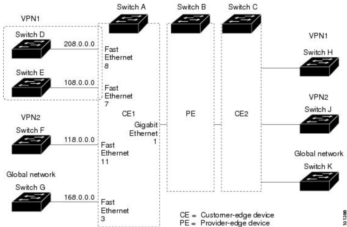
Figure 14: Multi-VRF CE Configuration Example
