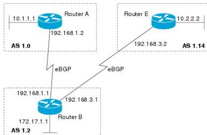
Figure 10: BGP Peers Using 4-Byte Autonomous System Numbers in Asdot Format
