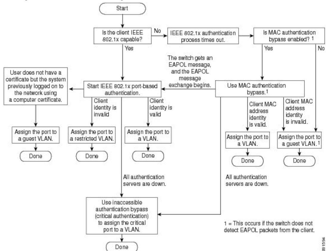
Figure 34: Authentication Flowchart
