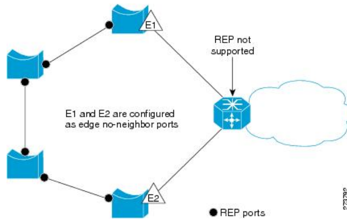
Figure 23: Edge No-Neighbor Ports
