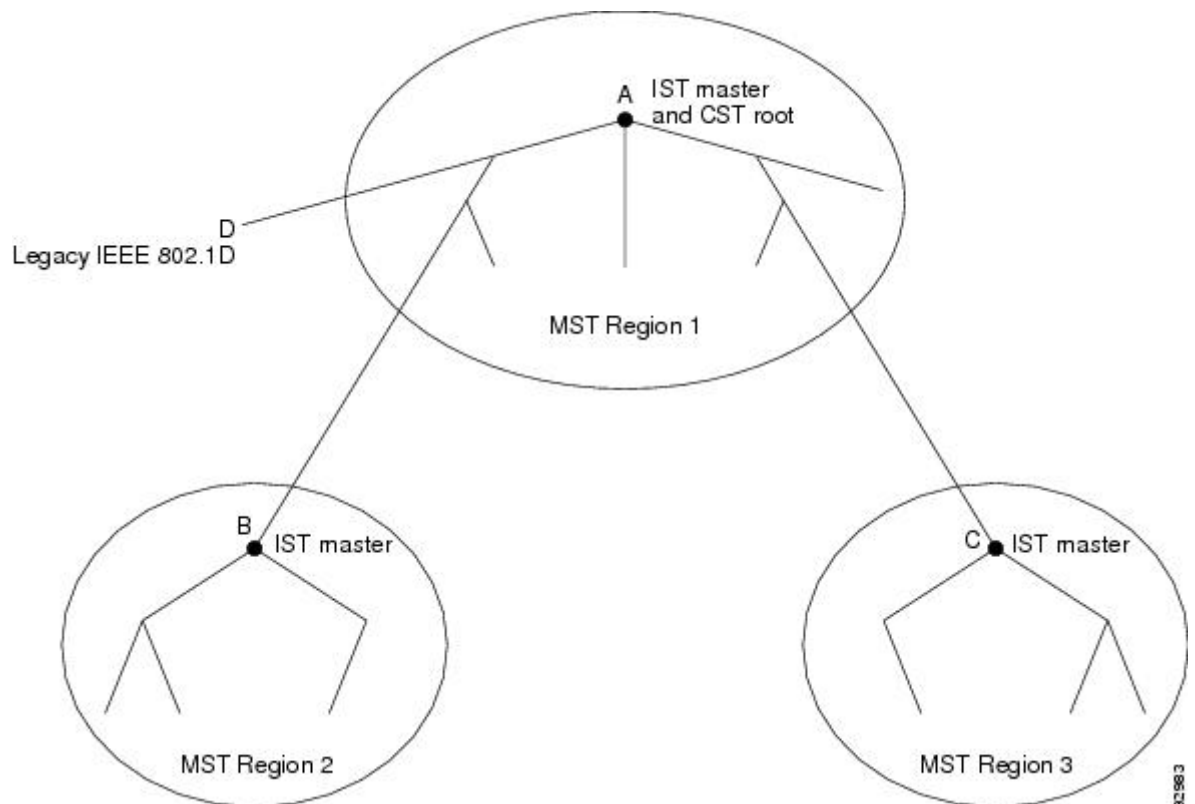
Figure 4: MST Regions, CIST Masters, and CST Root
